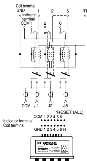
Latching type
