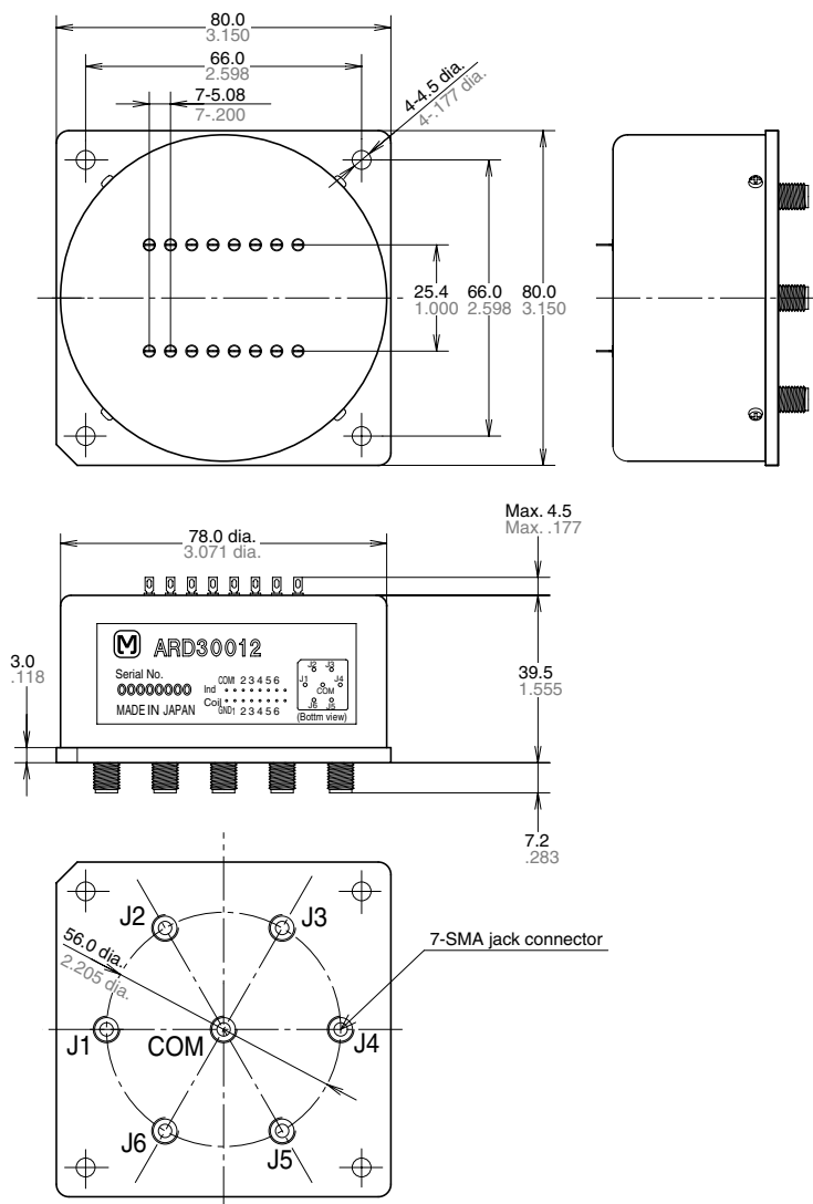
Latching type
