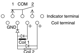
Latching
