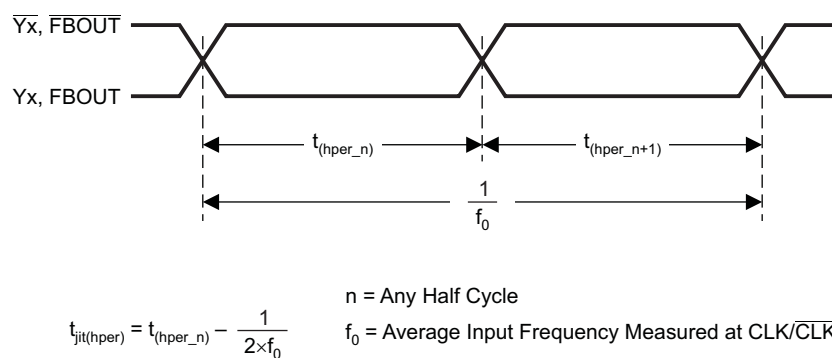
Figure 8. Half-Period Jitter
