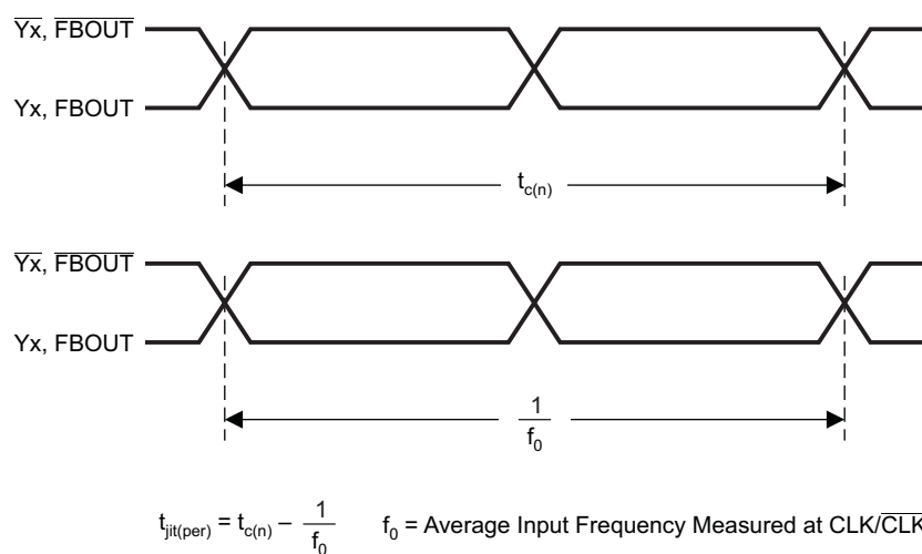
Figure 7. Period Jitter
