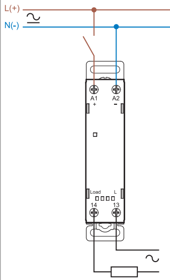
Single-phase connection (77.x5)
