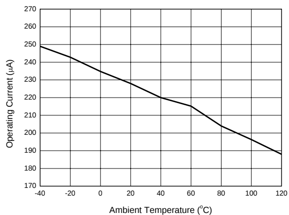
Figure 5. Operating Current vs. Ambient Temperature
