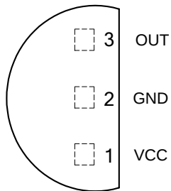
Z Package (TO-92 Bulk Packing)
