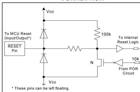
FIGURE 3-4: RESET PIN INTERNAL CONNECTION
