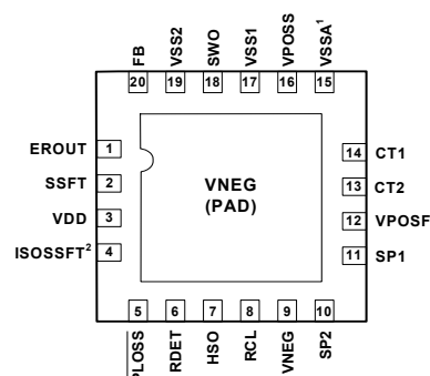
5 x 5 mm QFN (Top View)
