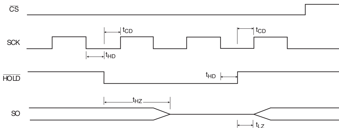
Figure 11. HOLD Timing
