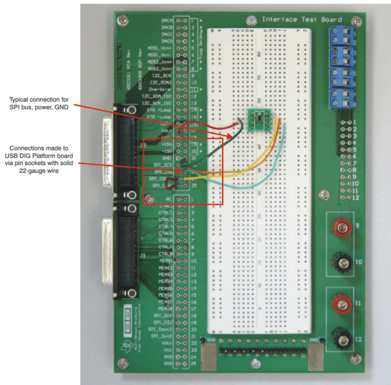
Figure 6. Interface Test Board Signal Connections
