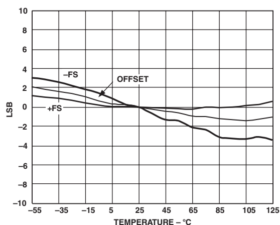
TPC 15. +FS, Offset, and -FS vs. Temperature
