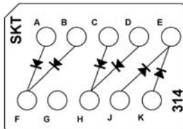
CTJ420E314 Six 1N4007 Diodes
