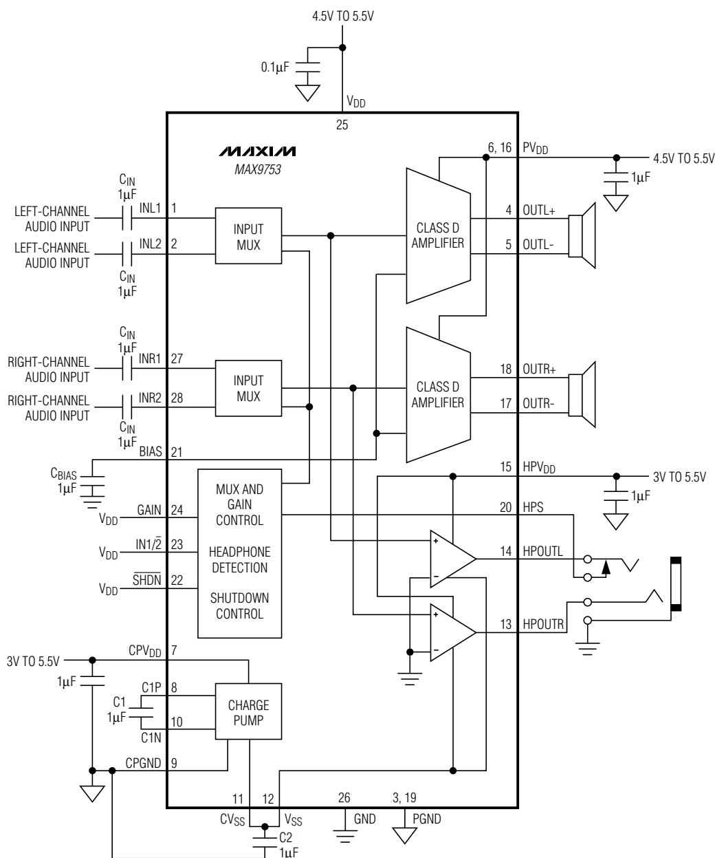
MAX9753 Functional Diagram
