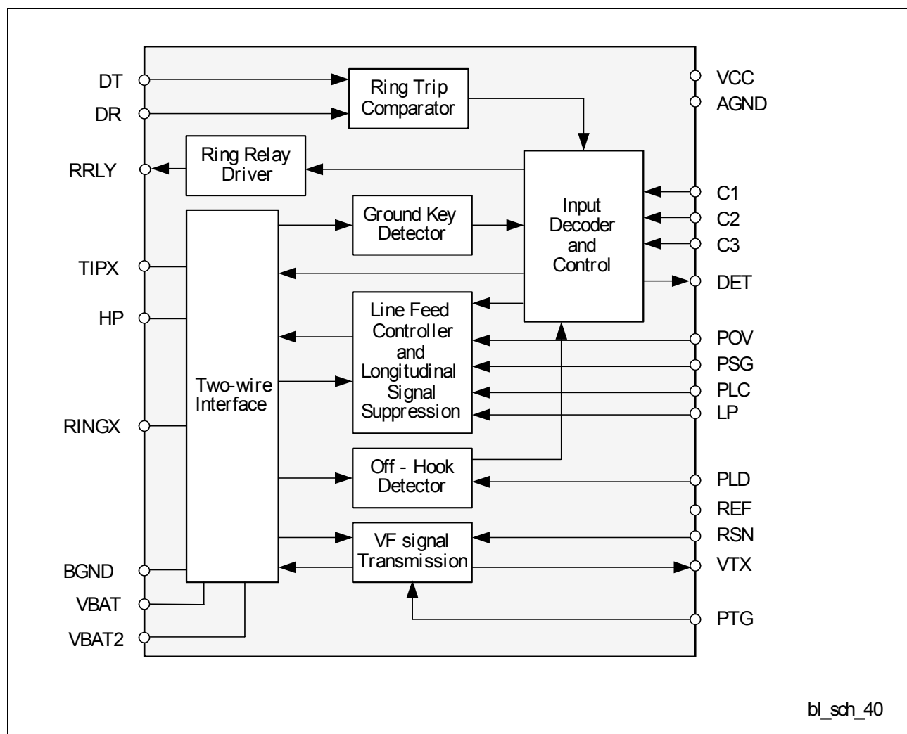
Figure 1 Block Diagram
