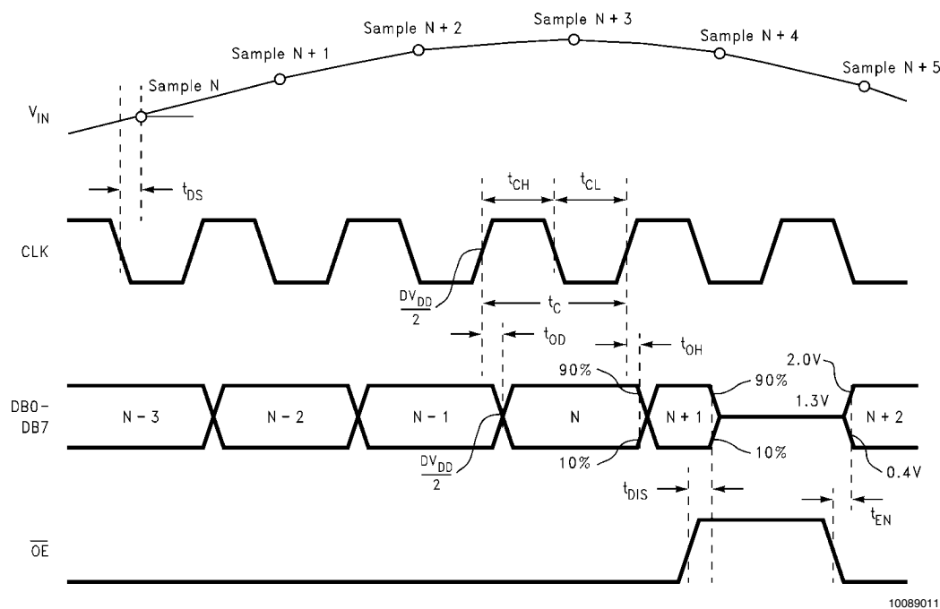
FIGURE 1. Timing Diagram
