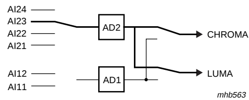
Fig 46. Mode 4 CVBS (automatic gain)
