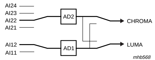
Fig 49. Mode 7 Y+ C (gain channel 2 adjusted via GAI2)
