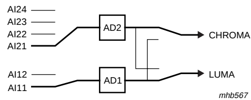
Fig 48. Mode 6 Y+ C (gain channel 2 adjusted via GAI2)
