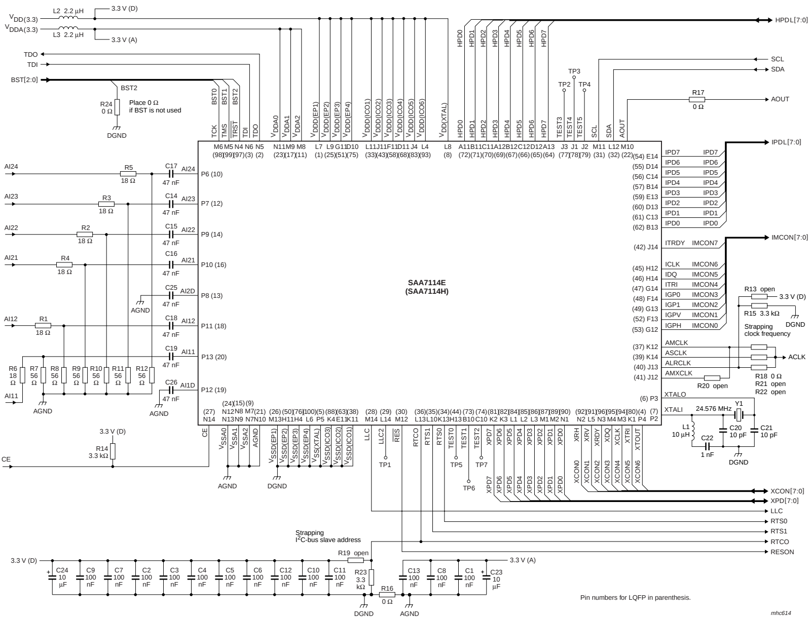
Fig 53. Application example with 24.576 MHz crystal
