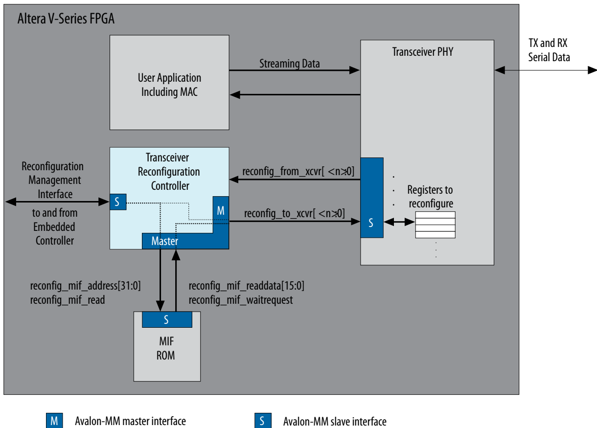
Figure 16-1: Transceiver Reconfiguration Controller
