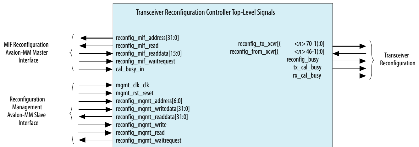
Figure 16-2: Top-Level Signals of the Transceiver Reconfiguration Controller
