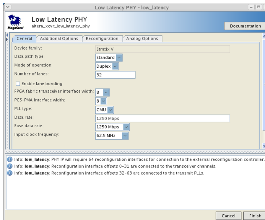
Figure 16-9: Low Latency Transceiver PHY Example
