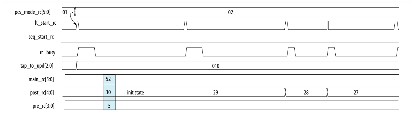
Figure 4-5: Transition from Auto Negotiation to Link Training Mode
