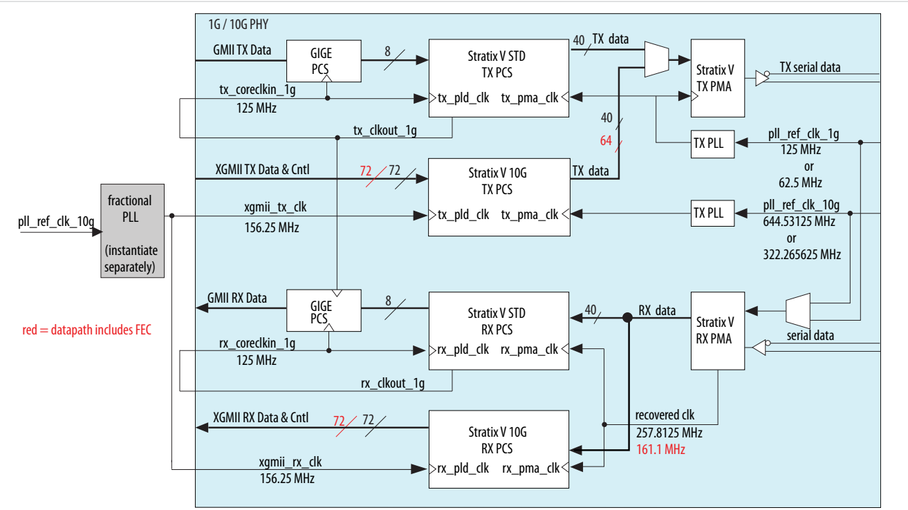
Figure 4-12: Clocks for Standard and 10G PCS and TX PLLs
