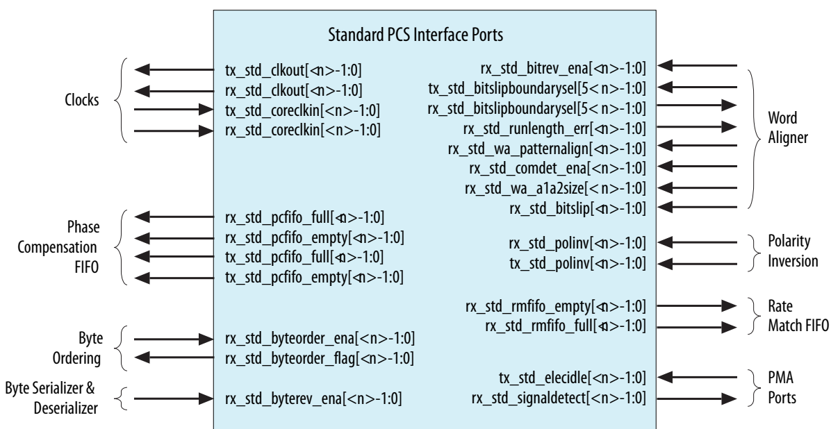
Figure 14-6: Standard PCS Interfaces
