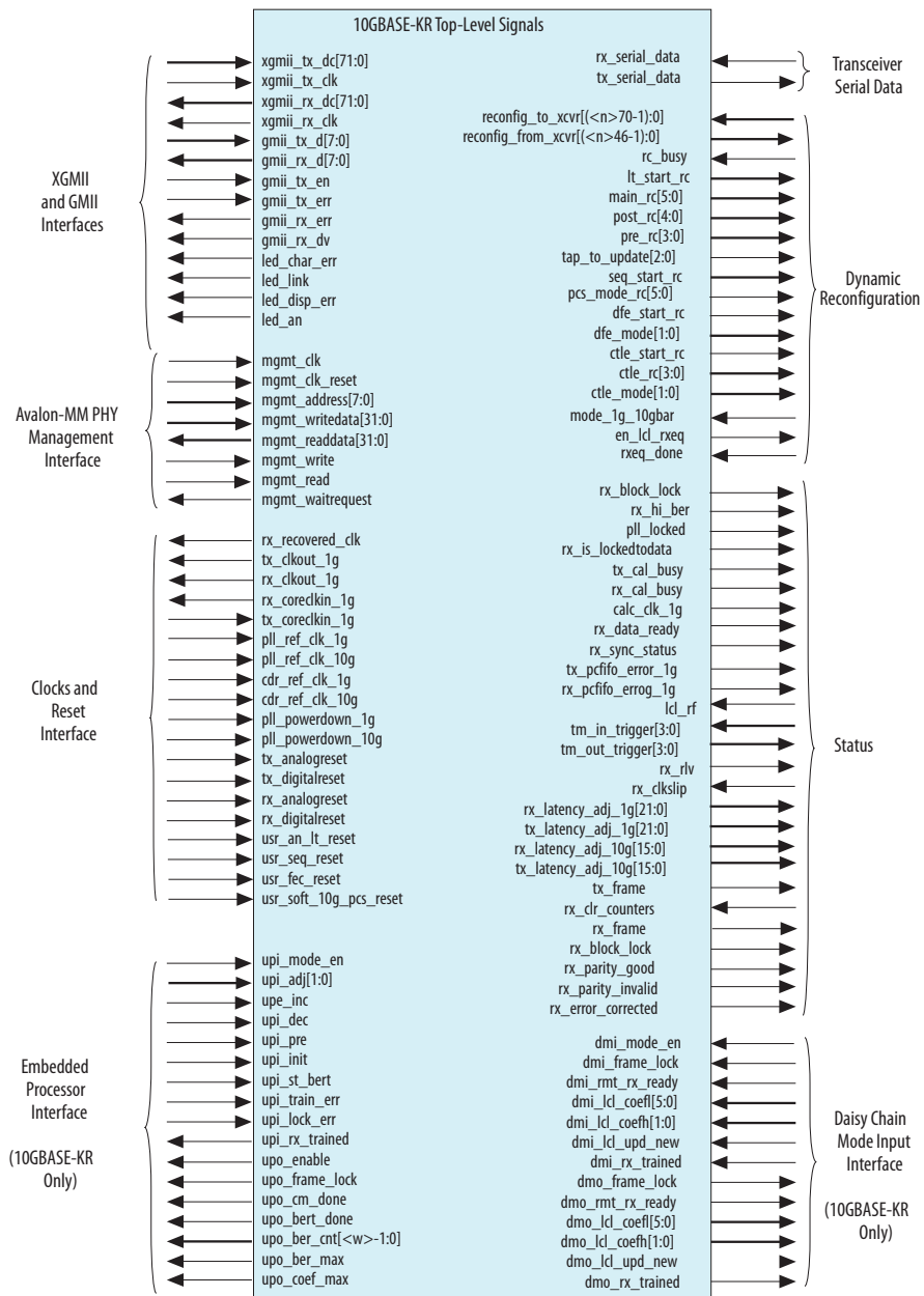
Figure 4-11: 10GBASE-KR Top-Level Signals
