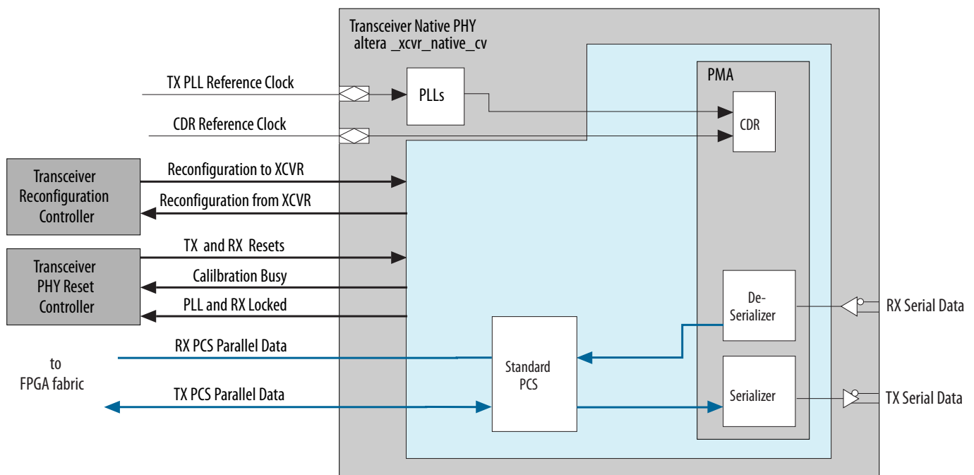
Figure 15-1: Cyclone Native Transceiver PHY IP Core
