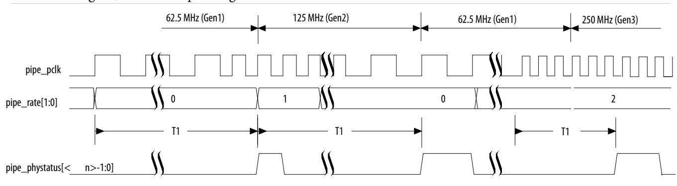
Figure 8-4: Rate Switch from Gen1 to Gen2 Timing Diagram
