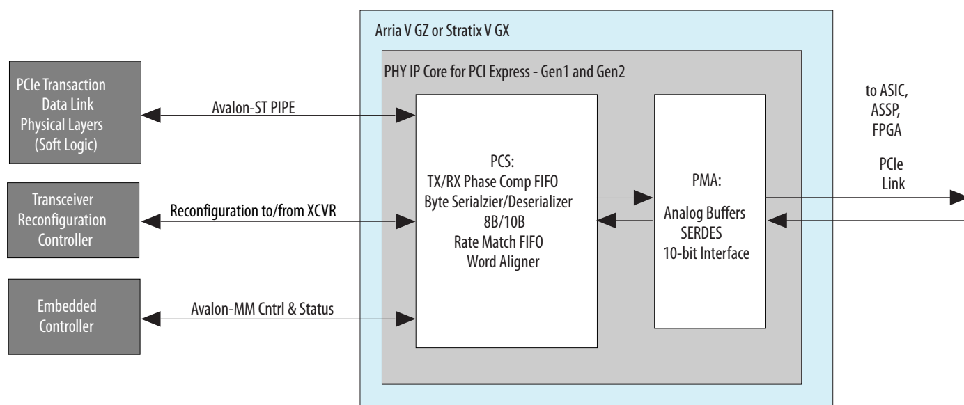
Figure 8-2: Gen1 and Gen2 PCI Express PHY (PIPE) with Hard IP PCS and PMA in Arria V GZ and Stratix V GX Devices
