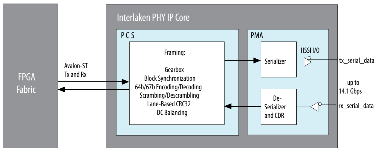
Figure 7-1: Interlaken PHY IP Core
