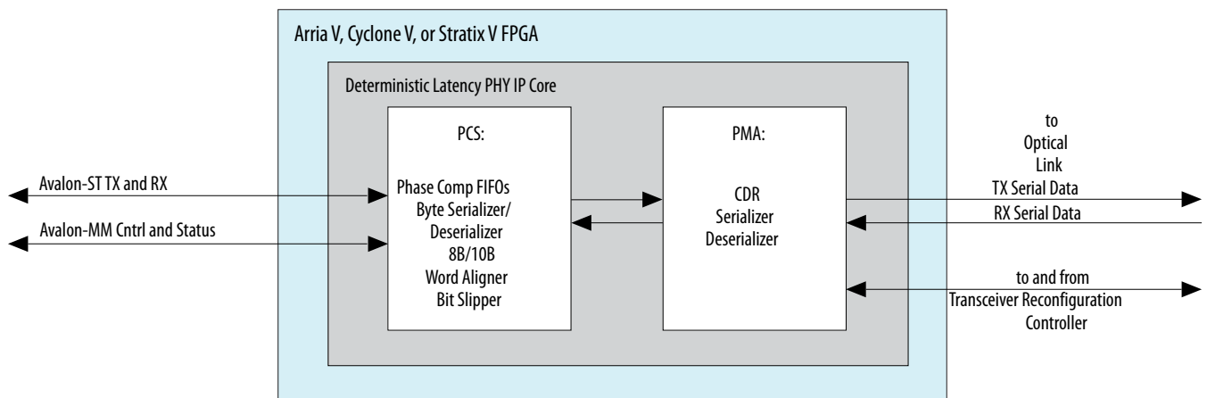
Figure 11-1: Deterministic Latency PHY IP Core
