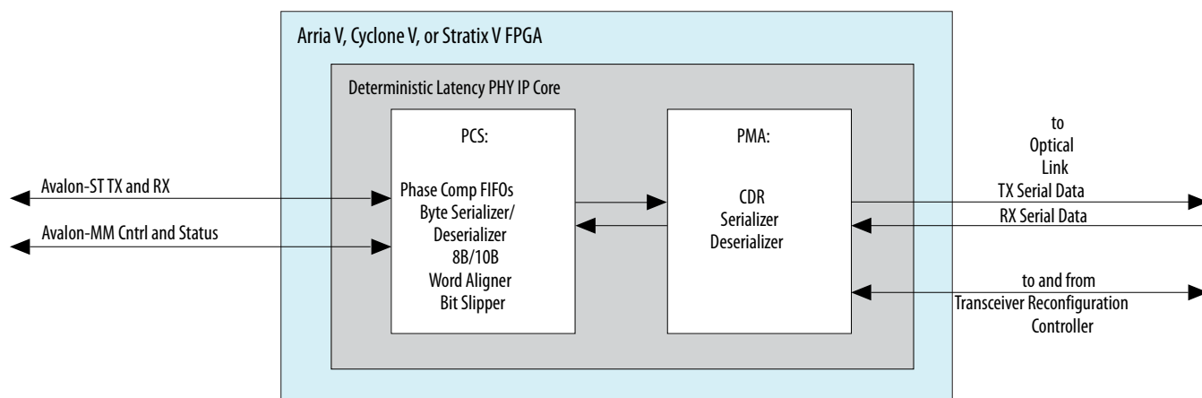
Figure 9-1: Custom PHY IP Core
