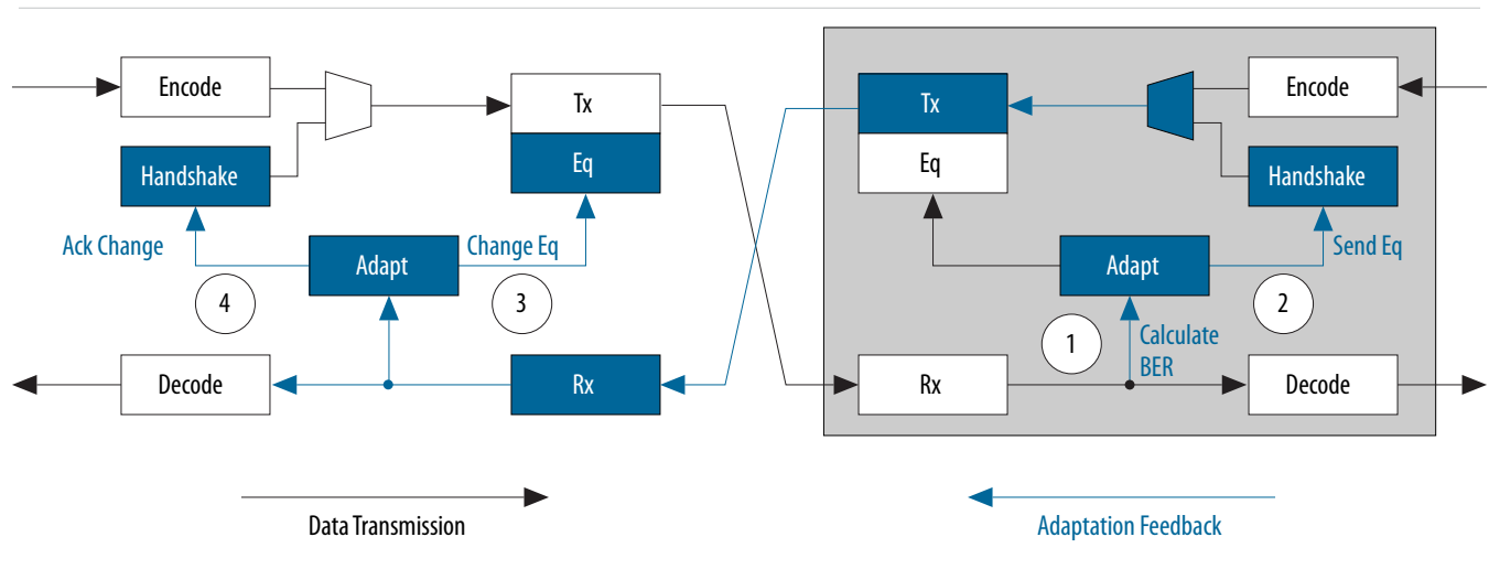
Figure 4-3: TX Equalization for Link Partners
