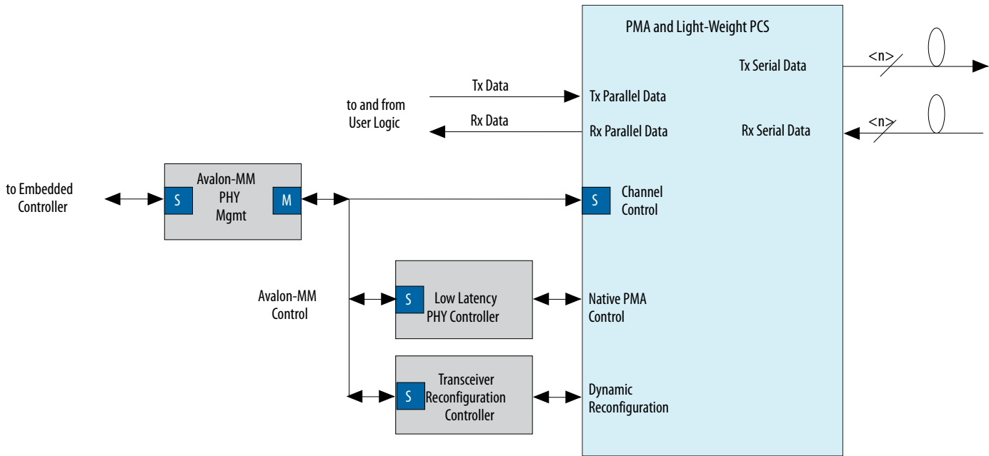
Figure 10-3: PMA Top-Level Modules
