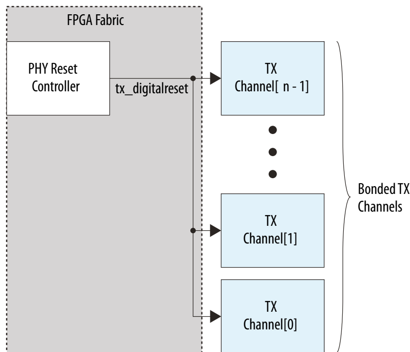
Figure 17-3: Physical Routing Delay Skew in Bonded Channels
