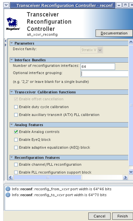
Figure 16-10: Transceiver Reconfiguration Controller Interface Bundles
