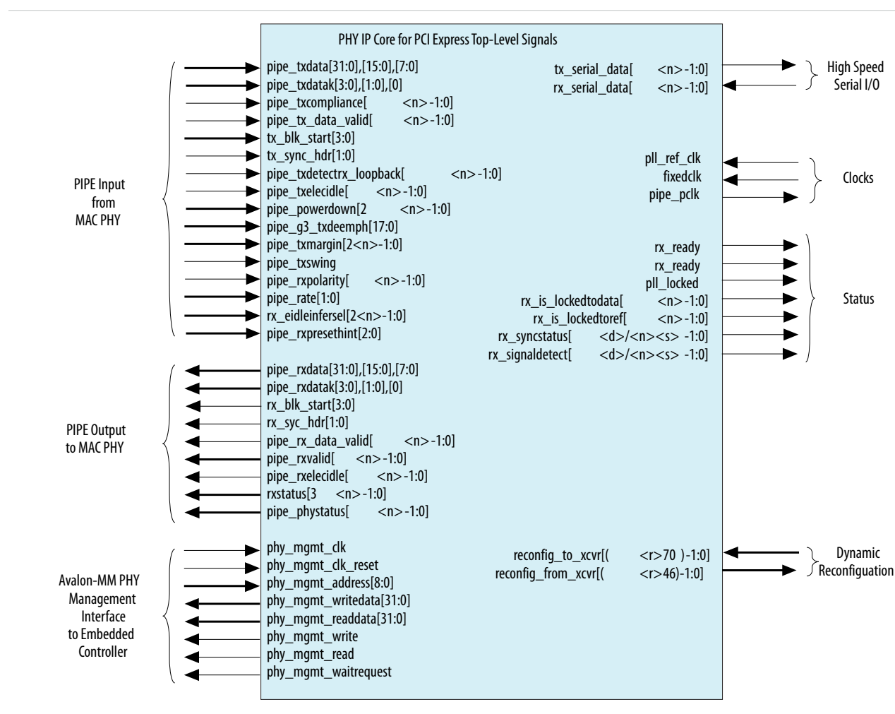
Figure 8-3: Top-Level Signals of the PHY IP Core for PCI Express
