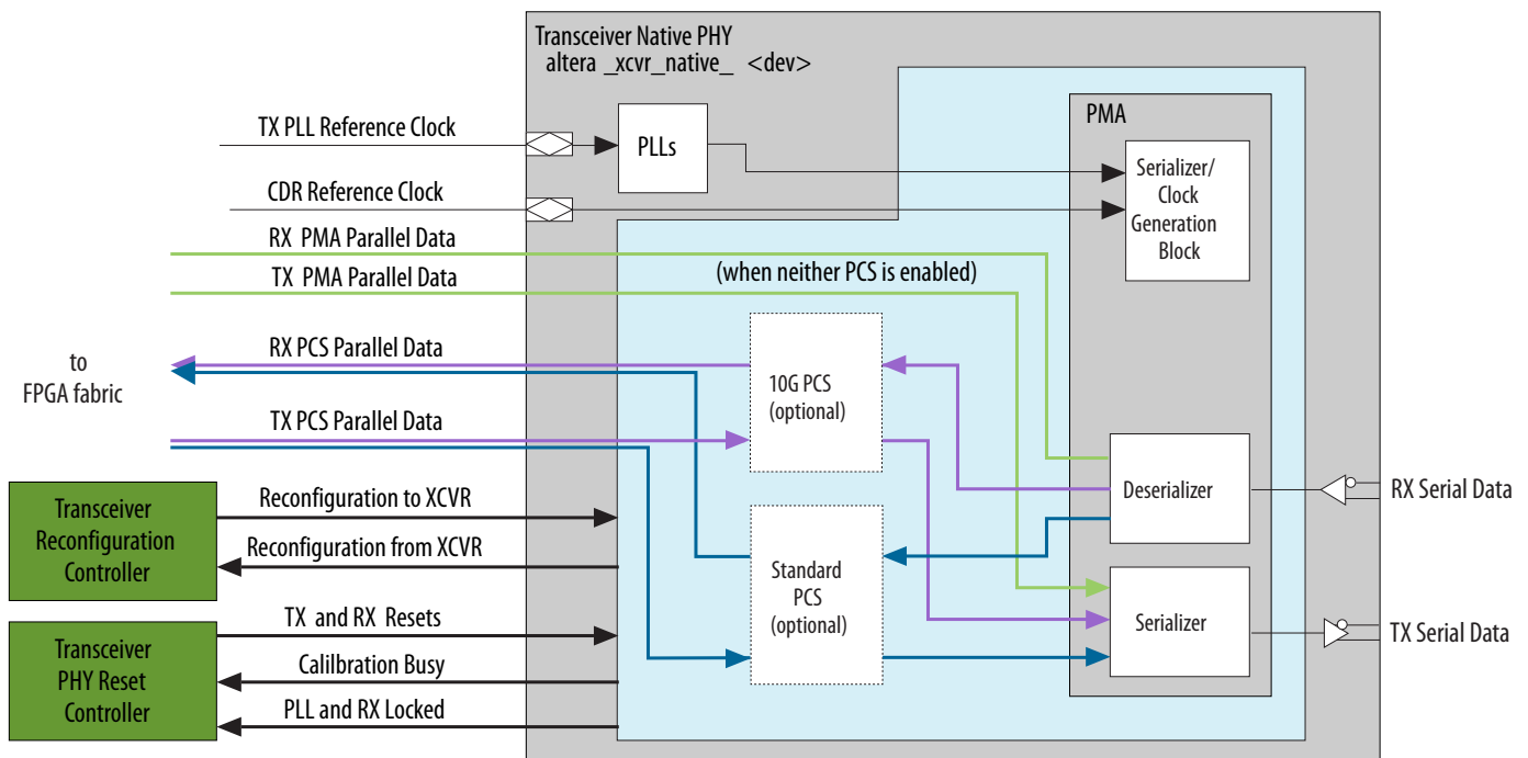
Figure 12-1: Stratix V Native Transceiver PHY IP Core
