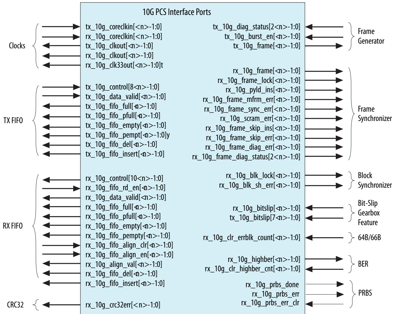
Figure 14-7: Arria V Native PHY 10G PCS Interfaces
