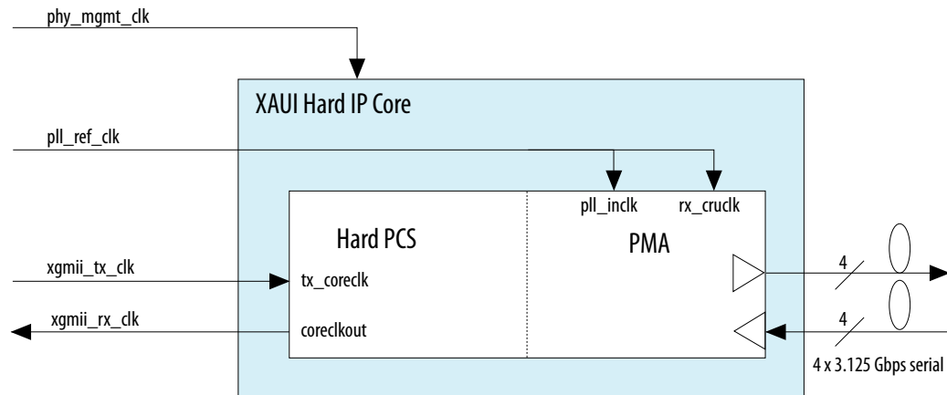
Figure 6-9: Clock Inputs and Outputs for IP Core with Soft PCS
