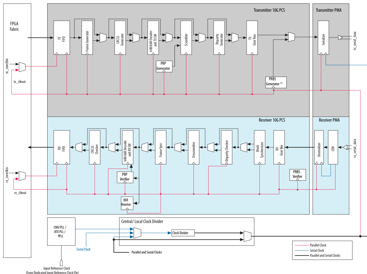
Figure 12-4: The 10G PCS datapath
