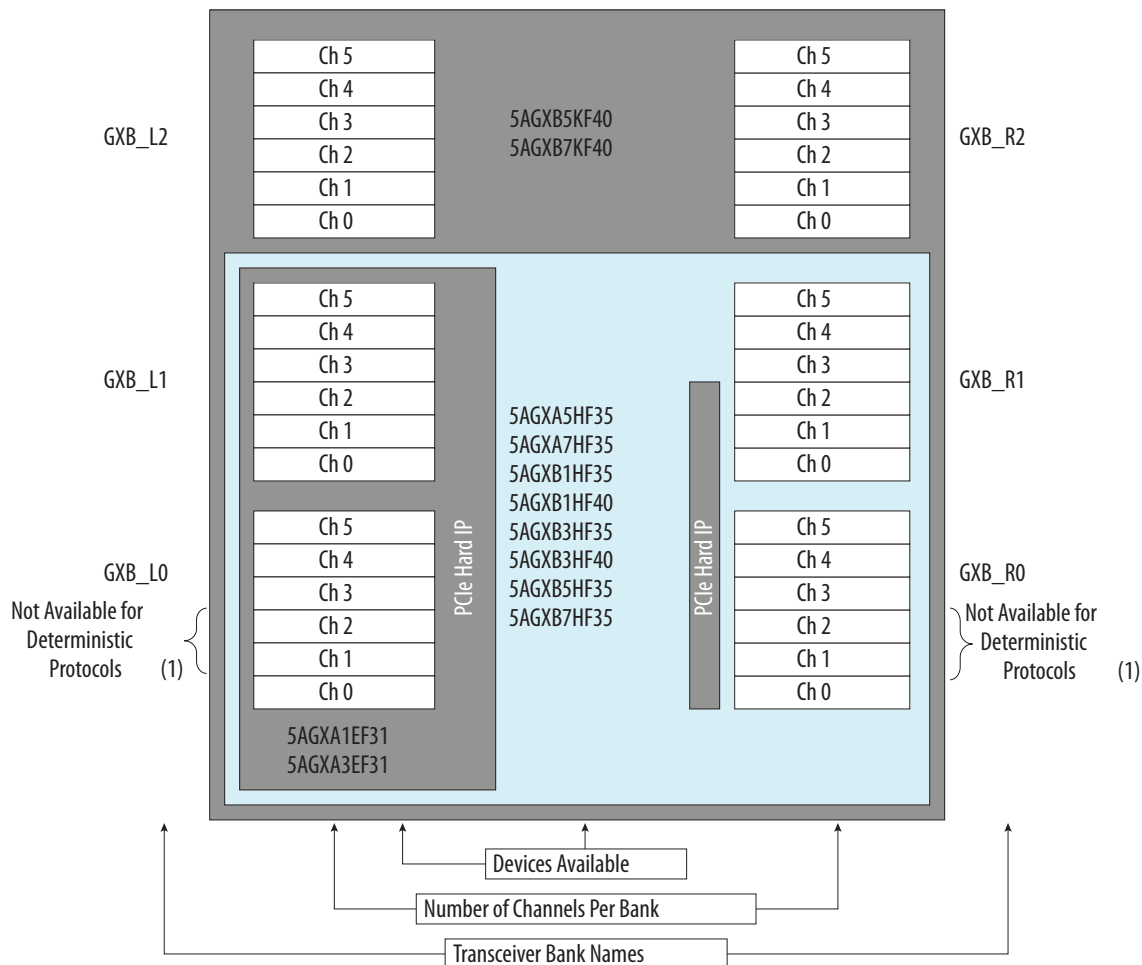
Figure 11-5: Channel Placement and Available Channels in Arria V Devices
