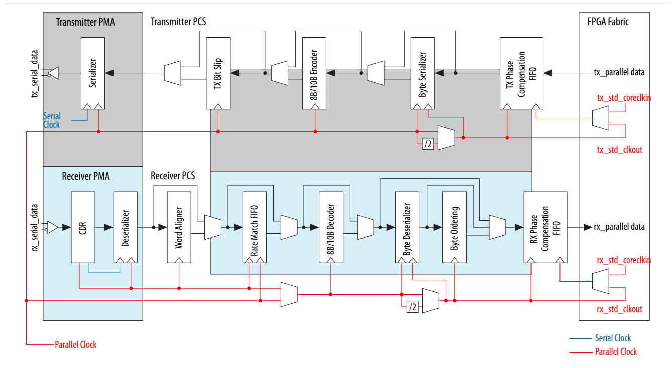
Figure 13-2: The Standard PCS Datapath
