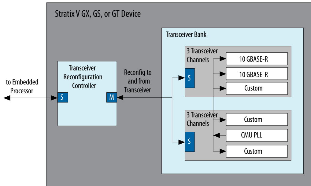
Figure 16-14: PLL Shared by Multiple Transceiver PHY IP Cores in a Single Transceiver Bank
