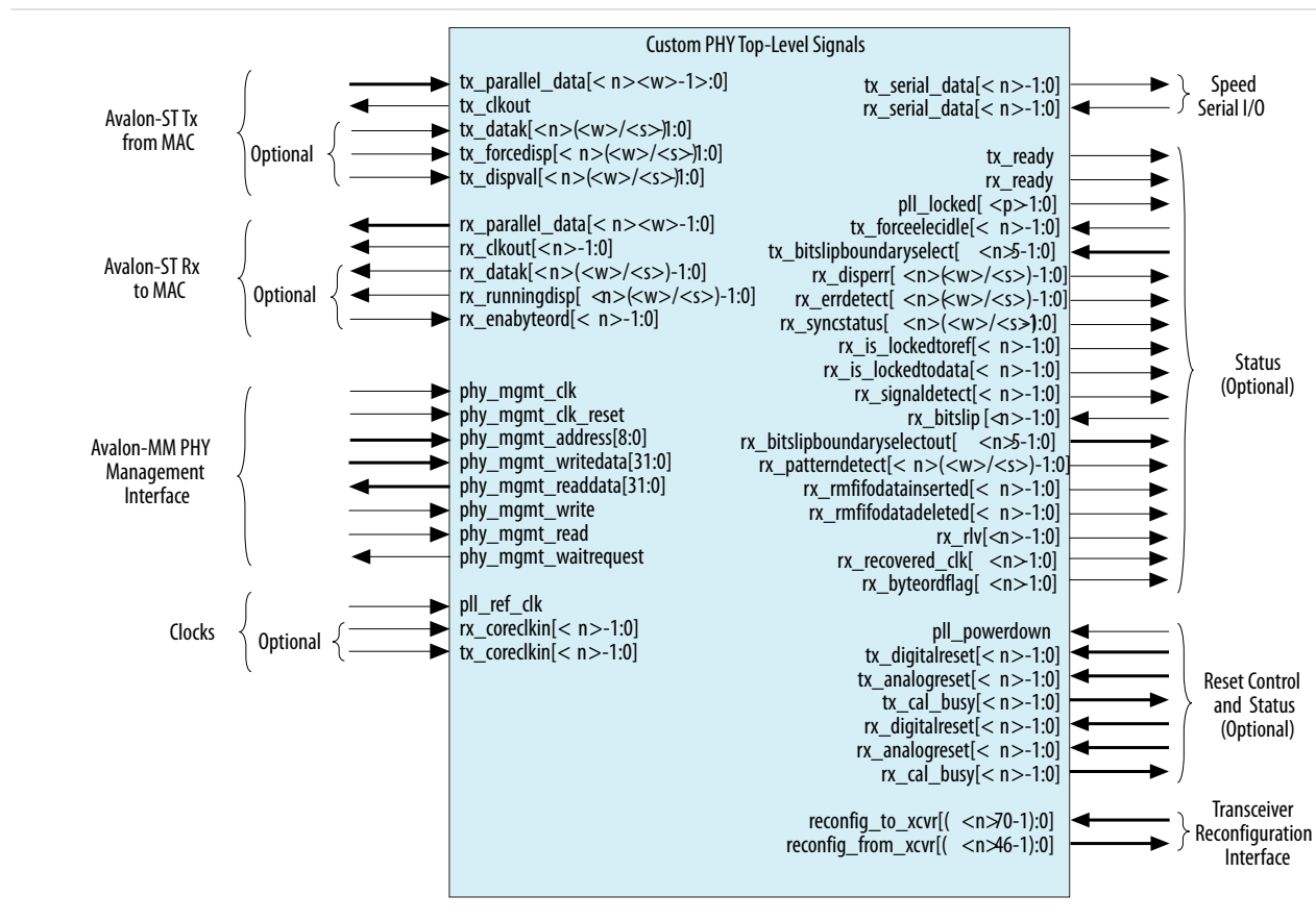
Figure 9-3: Custom PHY Interfaces
