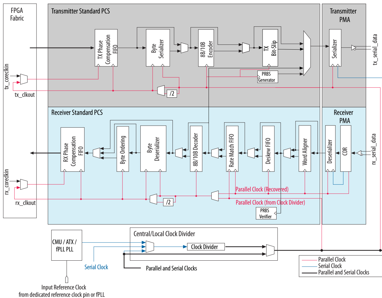
Figure 12-3: The Standard PCS Datapath
