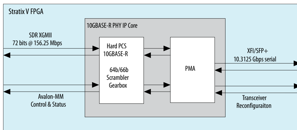
Figure 10-1: Low Latency PHY IP Core-Stratix V Devices
