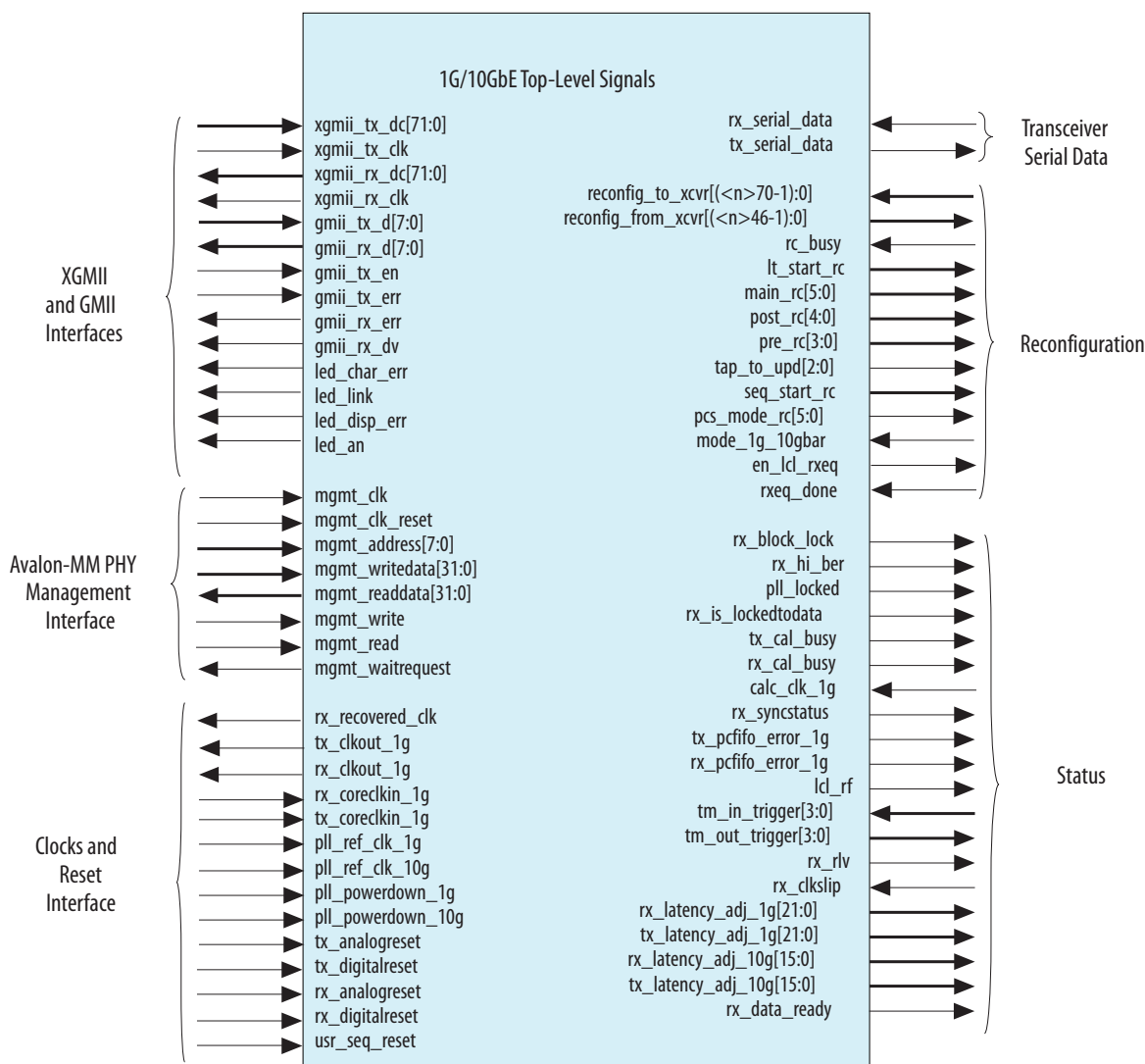
Figure 5-2: 1G/10GbE PHY Top-Level Signals
