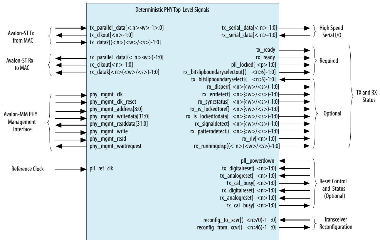
Figure 11-3: Deterministic Latency PHY Top-Level Signals
