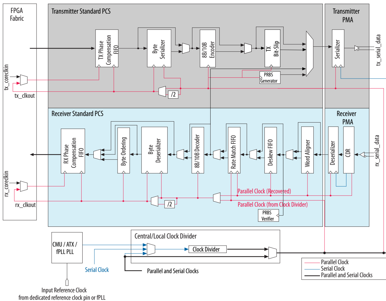
Figure 14-3: The Standard PCS Datapath
