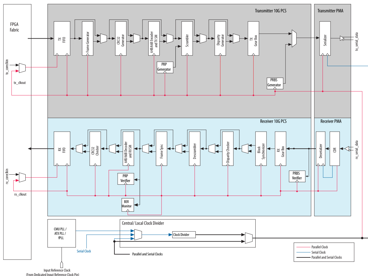
Figure 14-4: The 10G PCS datapath
