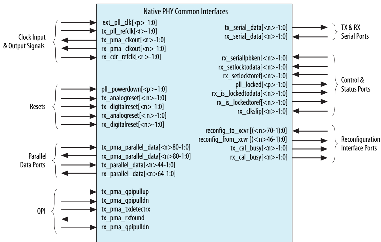
Figure 13-3: Common Interface Ports
