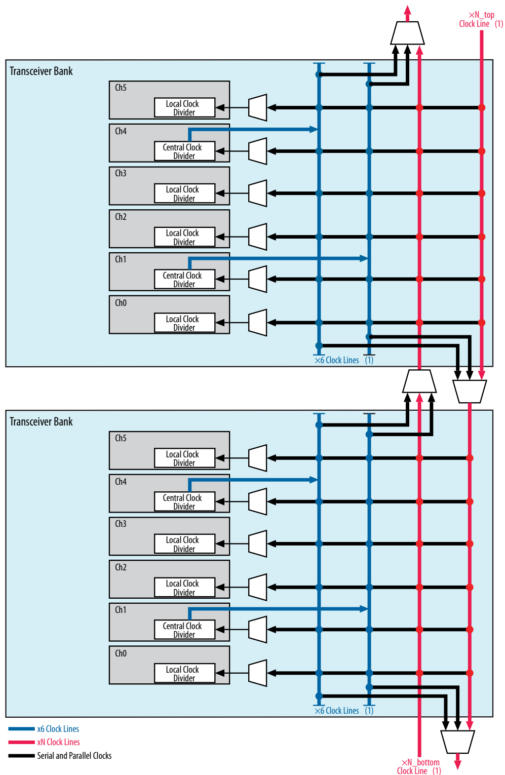
Figure 12-8: x6 and xN Routing of Clocks
