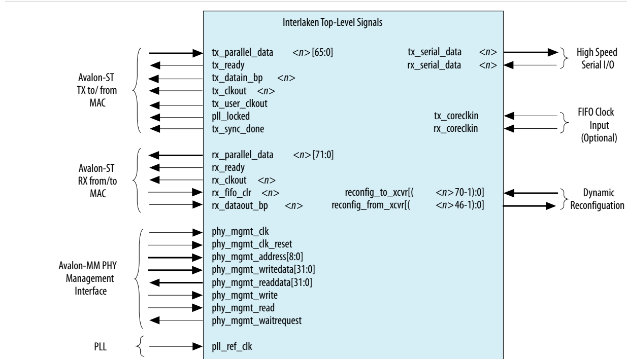
Figure 7-2: Top-Level Interlaken PHY Signals
