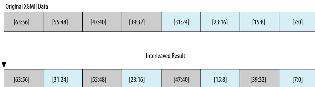
Figure 6-5: Interleaved SDR XGMII Data Mapping
