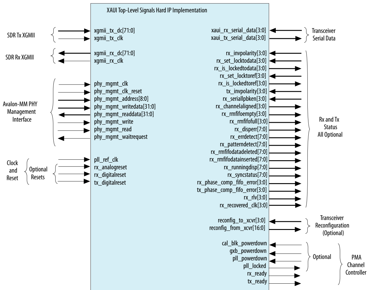
Figure 6-3: XAUI Top-Level Signals—Hard IP PCS and PMA
