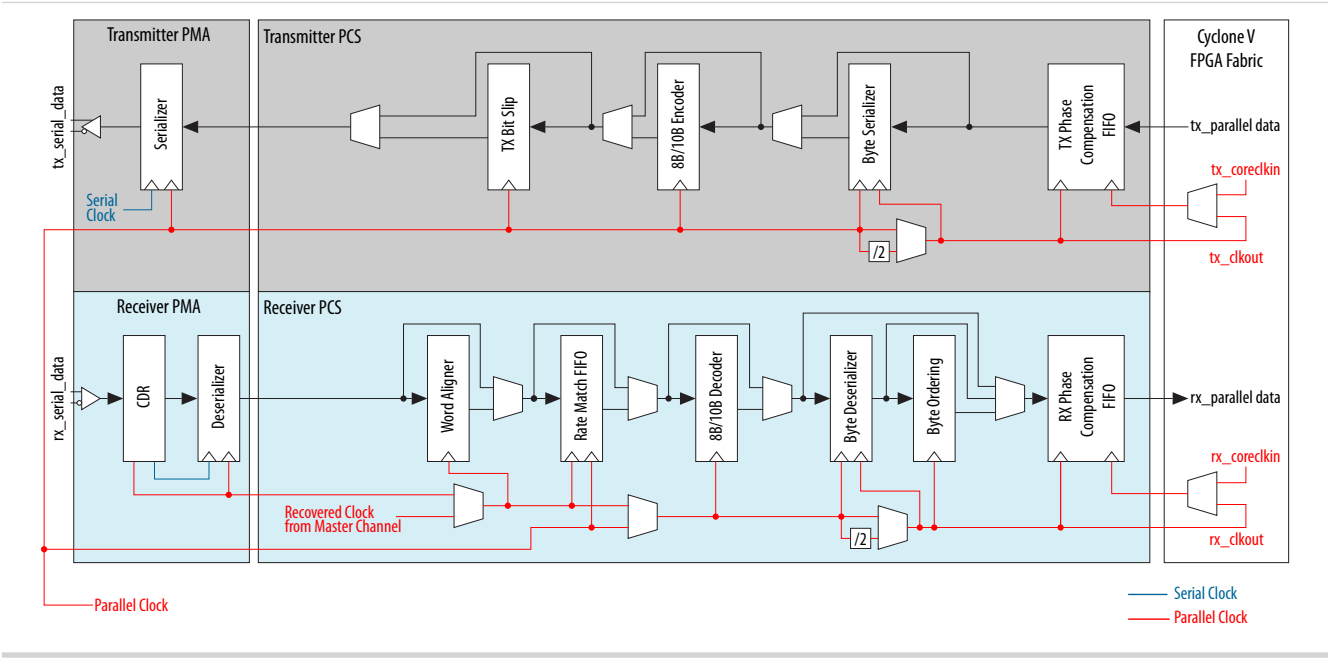
Figure 15-2: The Standard PCS Datapath
