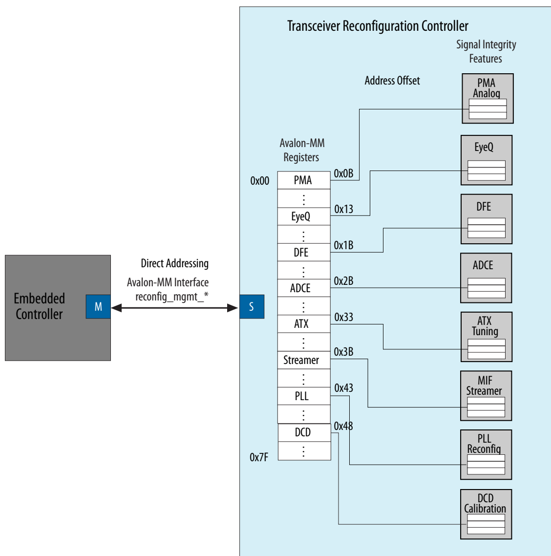
Figure 16-3: Memory Map of the Transceiver Reconfiguration Controller Registers
