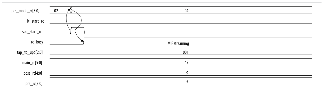
Figure 4-6: Transition from Link Training to Data Mode
