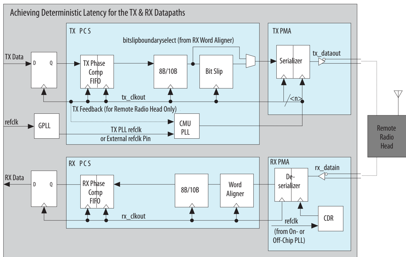
Figure 11-2: Achieving Deterministic Latency for the TX and RX Datapaths
