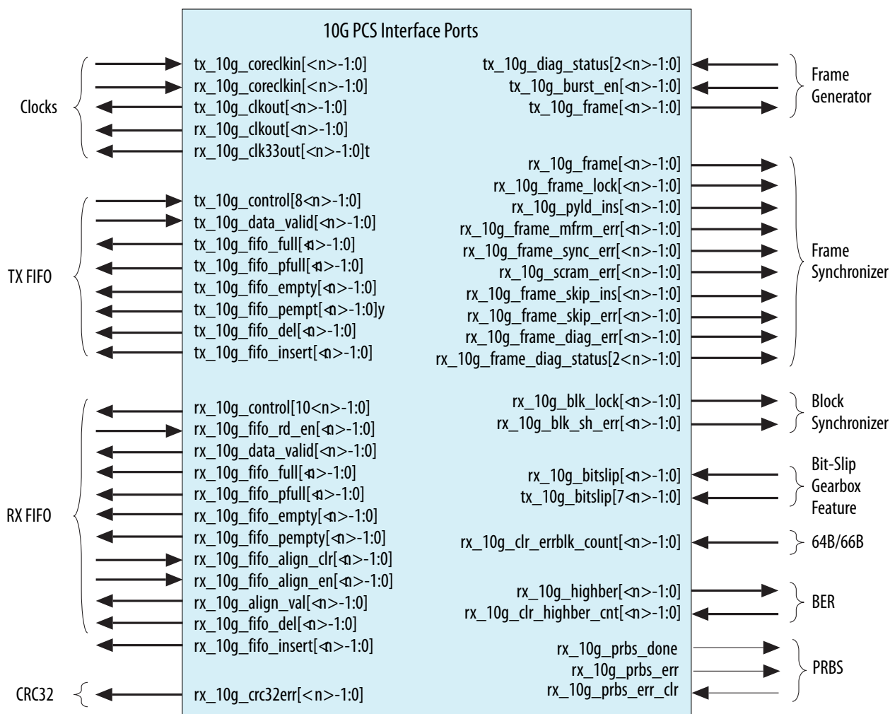
Figure 12-7: Stratix V Native PHY 10G PCS Interfaces
