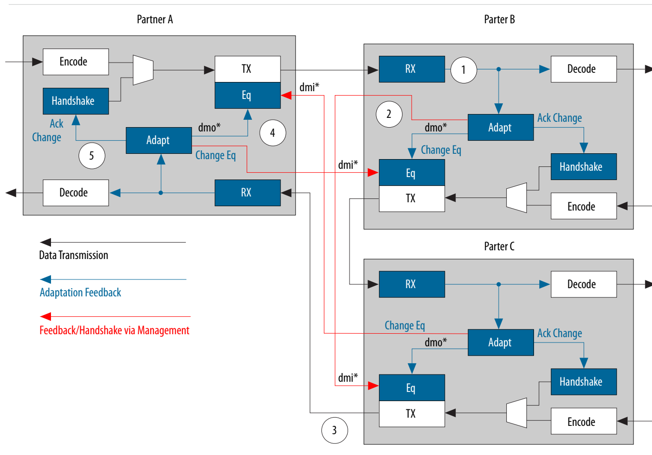
Figure 4-4: TX Equalization in Daisy-Chain Mode
