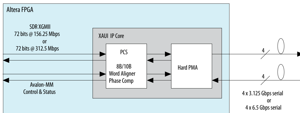
Figure 6-1: XAUI PHY IP Core
