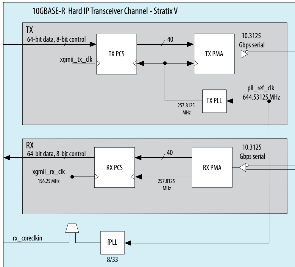
Figure 3-10: Stratix V Clock Generation and Distribution
