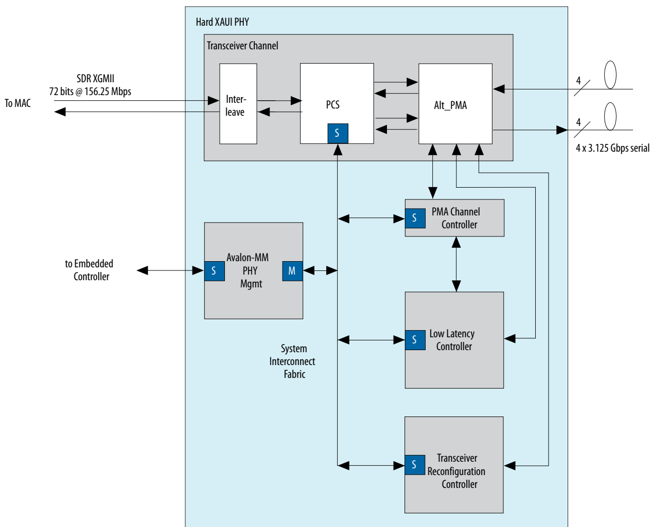
Figure 6-2: XAUI PHY with Internal Transceiver Reconfiguration Control
