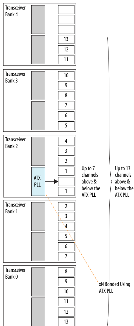
Figure 12-9: Channel Span for xN Bonded Channels
