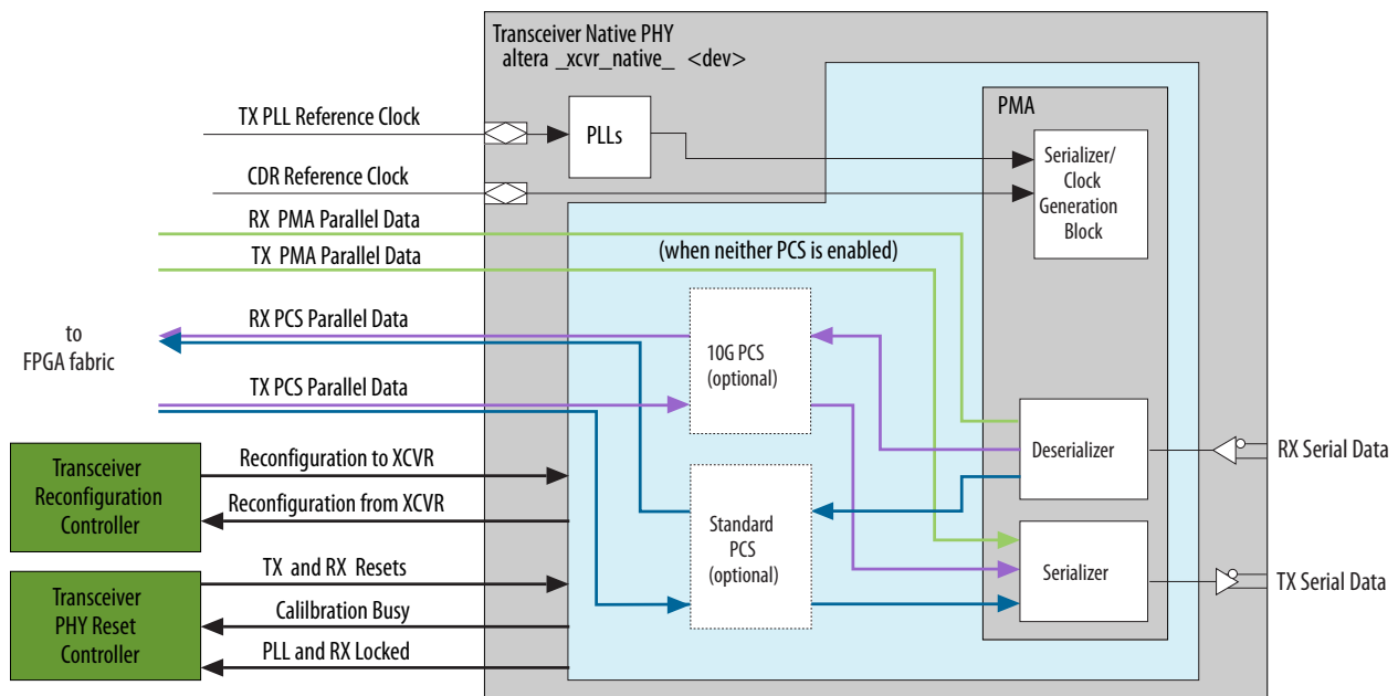
Figure 14-1: Arria V GZ Native Transceiver PHY IP Core
