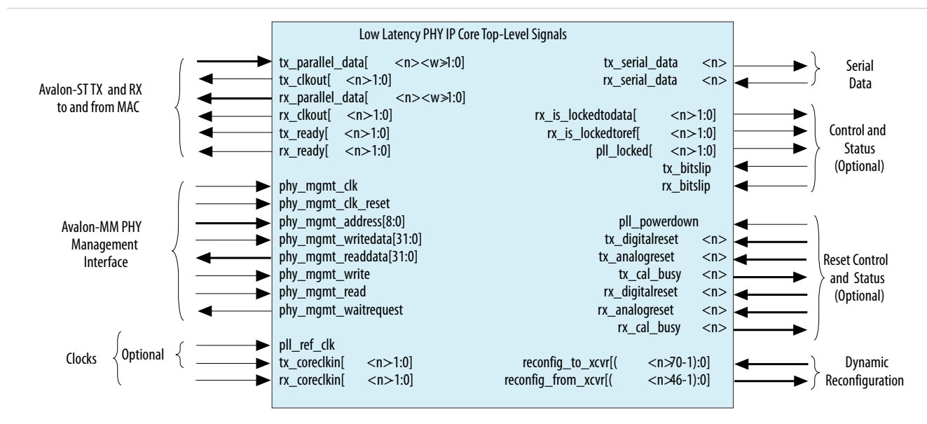
Figure 10-2: Top-Level Low Latency Signals
