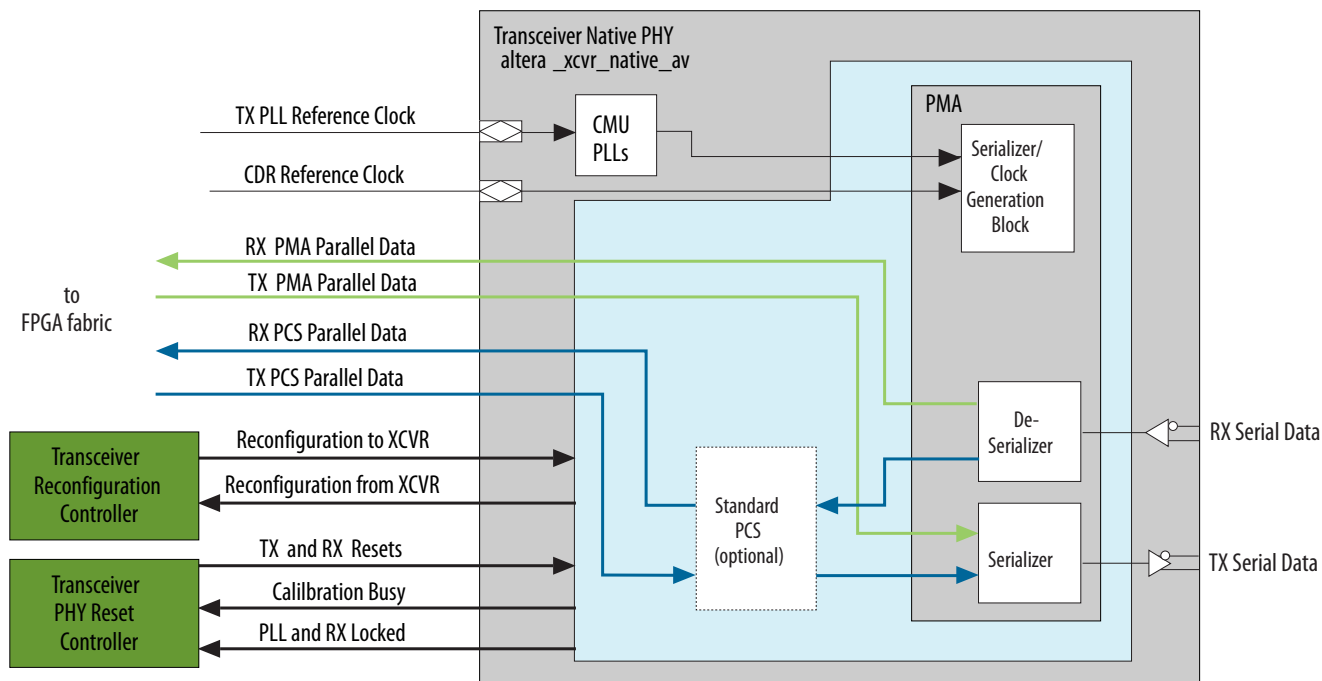
Figure 13-1: Arria Native Transceiver PHY IP Core
