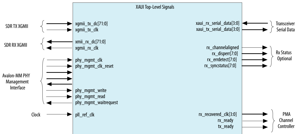
Figure 6-4: XAUI Top-Level Signals—Soft PCS and PMA
