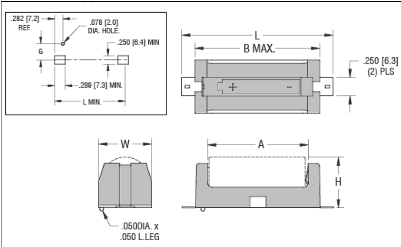
Thru-Hole Mount
