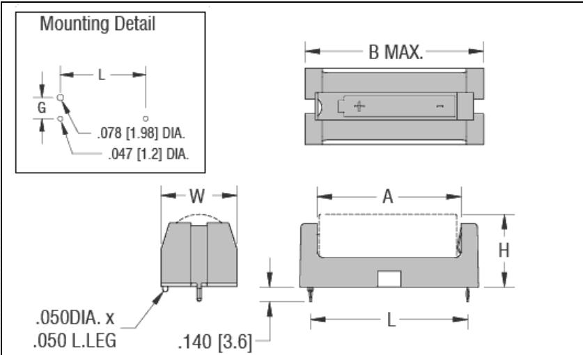
Thru-Hole Mount
