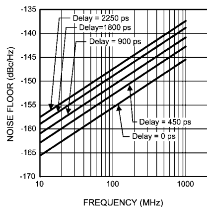
Delay Noise Floor (Adds to Output Noise Floor) (Notes 18, 19)
