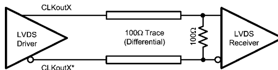
FIGURE 6. Differential LVDS Operation, DC Coupling
