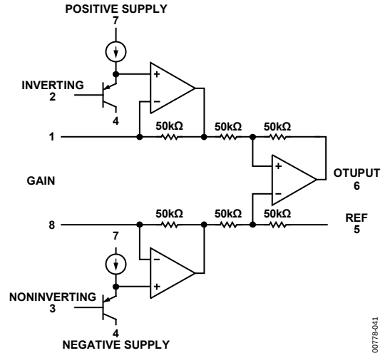
Figure 41. Simplified Schematic
