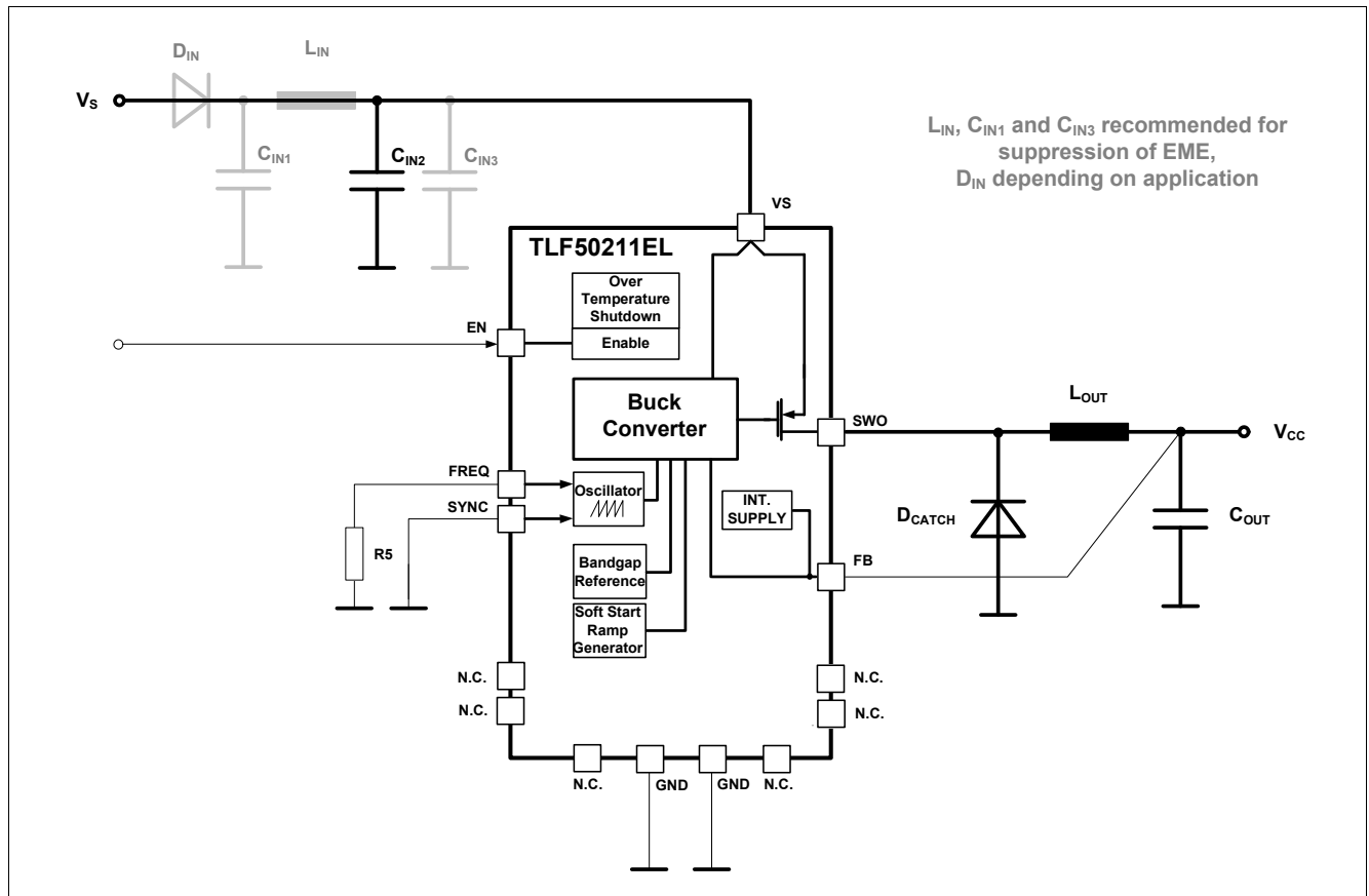
Figure 8 Application Diagram
