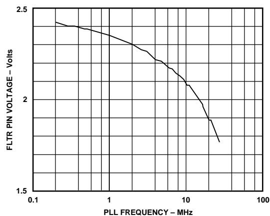
Figure 23. PLL Loop Voltage at FLTR ( K_{VCO} ) vs. Frequency
