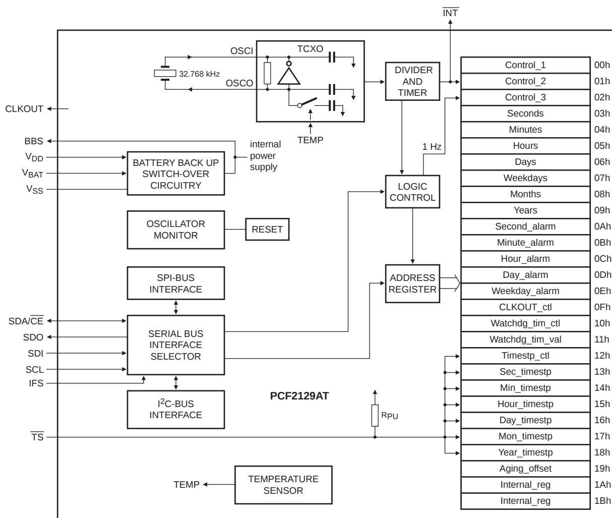
Fig 1. Block diagram of PCF2129AT
