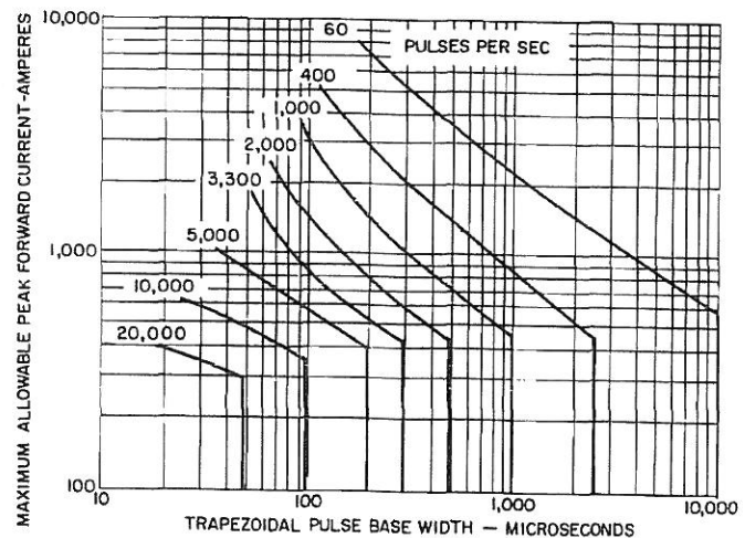
6. MAXIMUM ALLOWABLE PEAK FORWARD CURRENT, TRAPEZOIDAL WAVEFORM ( T_C = 90^\circ\text{C} ) DOUBLE SIDE COOLED
