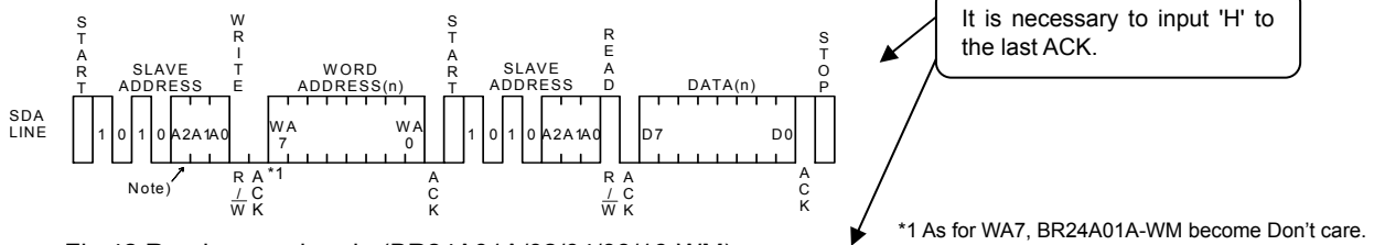
Fig.42 Random read cycle (BR24A01A/02/04/08/16-WM)
