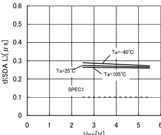
Fig.31 Noise removal valid time t(\text{SDA L})
