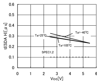
Fig.30 Noise removal valid time t(\text{SDA H})
