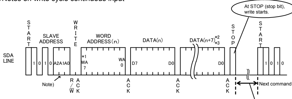
Fig.40 Page write cycle
