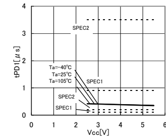
Fig.25 Output data delay time t_{PD1}
