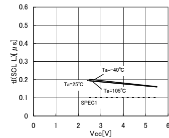
Fig.29 Noise removal valid time t(\text{SCL L})
