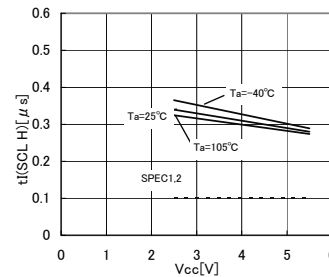
Fig.28 Noise removal valid time t(\text{SCL H})
