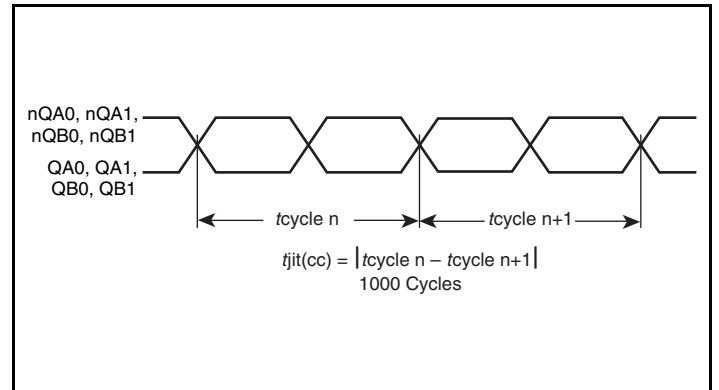
Cycle-to-Cycle Jitter
