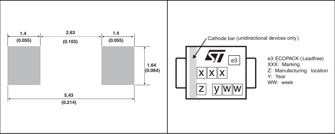
Figure 18. SMA footprint dimensions in millimeters (inches)
