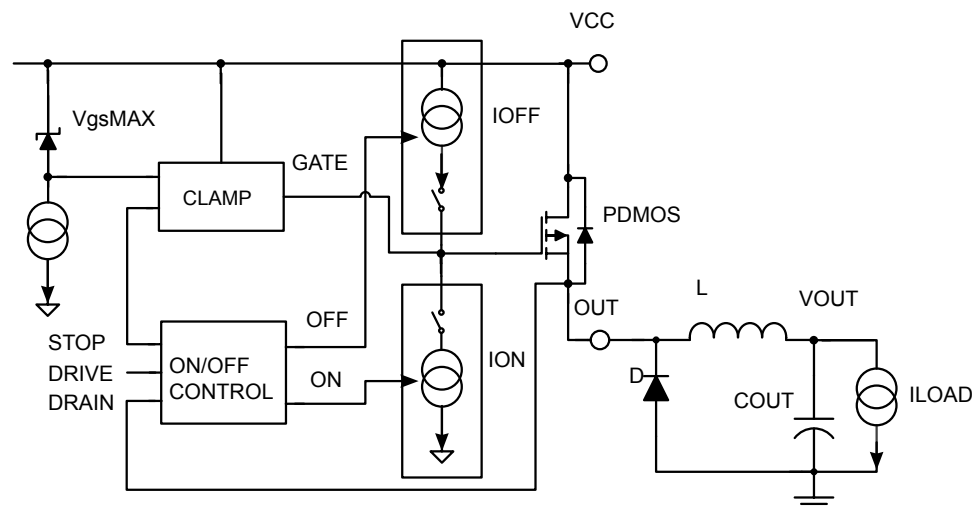
Figure 5. Driving circuitry
