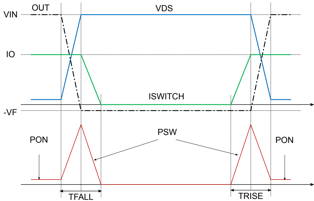
Figure 10. Switching losses
