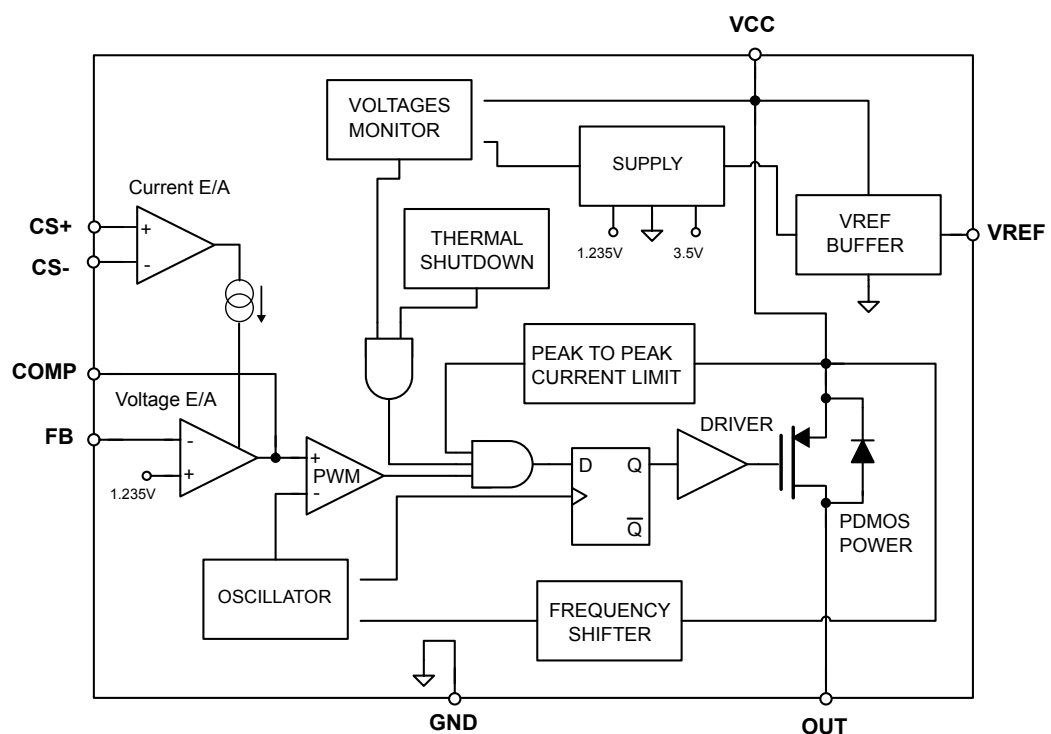
Figure 2. Block diagram
