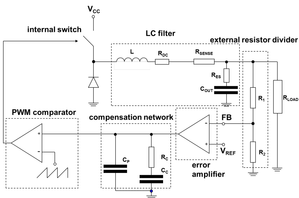
Figure 9. Constant current loop block diagramConstant current loop block diagram
