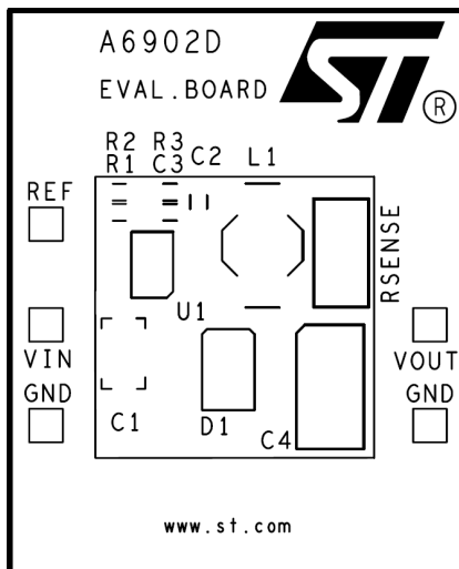
Figure 14. PCB layout (component side)
