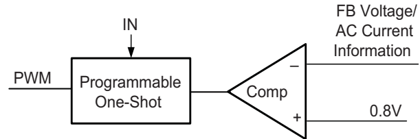
Figure 1. Simplified Control Schematic of AOZ1232-01
