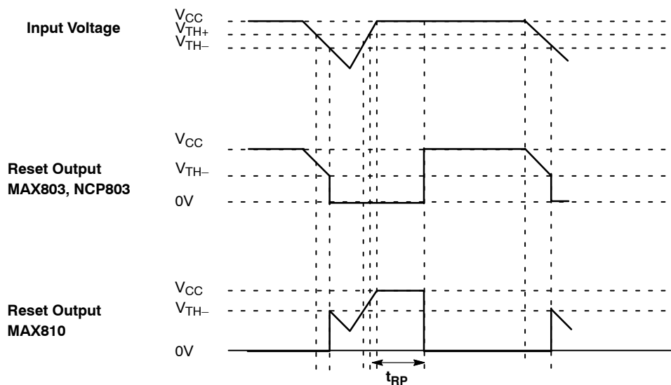
Figure 12. Timing Waveforms
