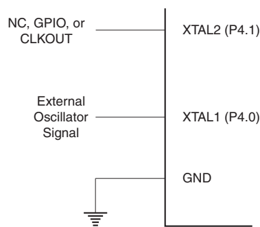
Figure 6-2. External Clock Drive Configuration
