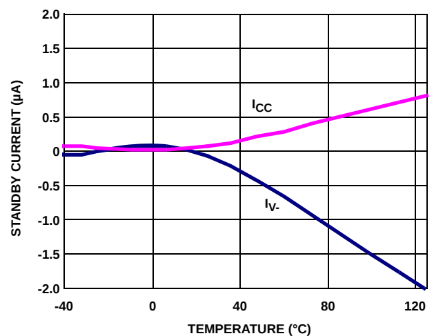
FIGURE 2. STANDBY I_{CC} and I_V vs TEMPERATURE
