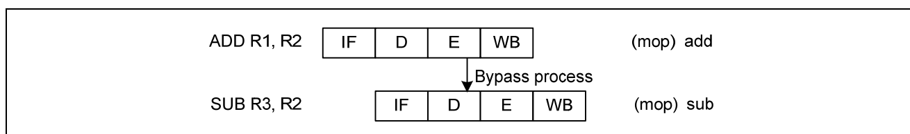
Figure 2.24 Bypass Process
