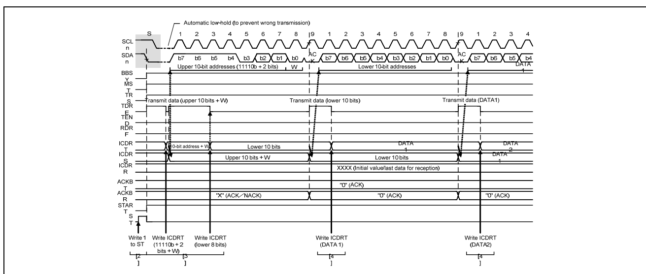
Figure 22.8 Master Transmit Operation Timing (2) (10-Bit Address Format)
