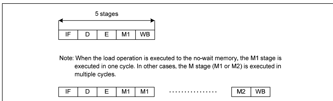
Figure 2.12 Load Operation
