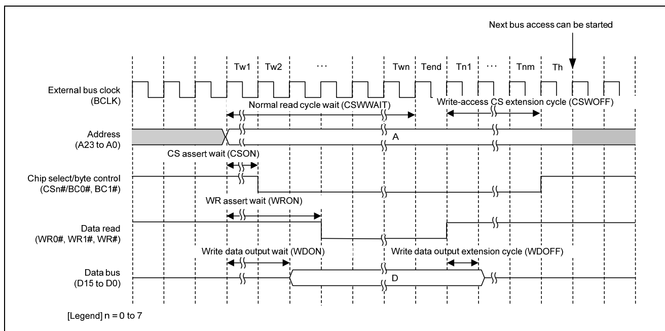
Figure 11.8 Bus Timing (Normal-Write Operation)
