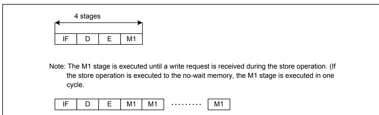
Figure 2.13 Store Operation
