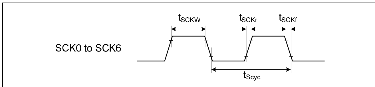
Figure 29.22 SCK Clock Input Timing
