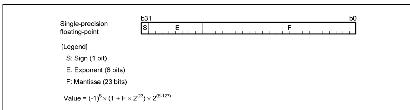
Figure 2.3 Floating-Point
