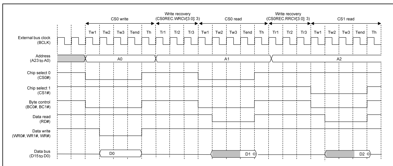
Figure 11.21 Example of Recovery Timing
