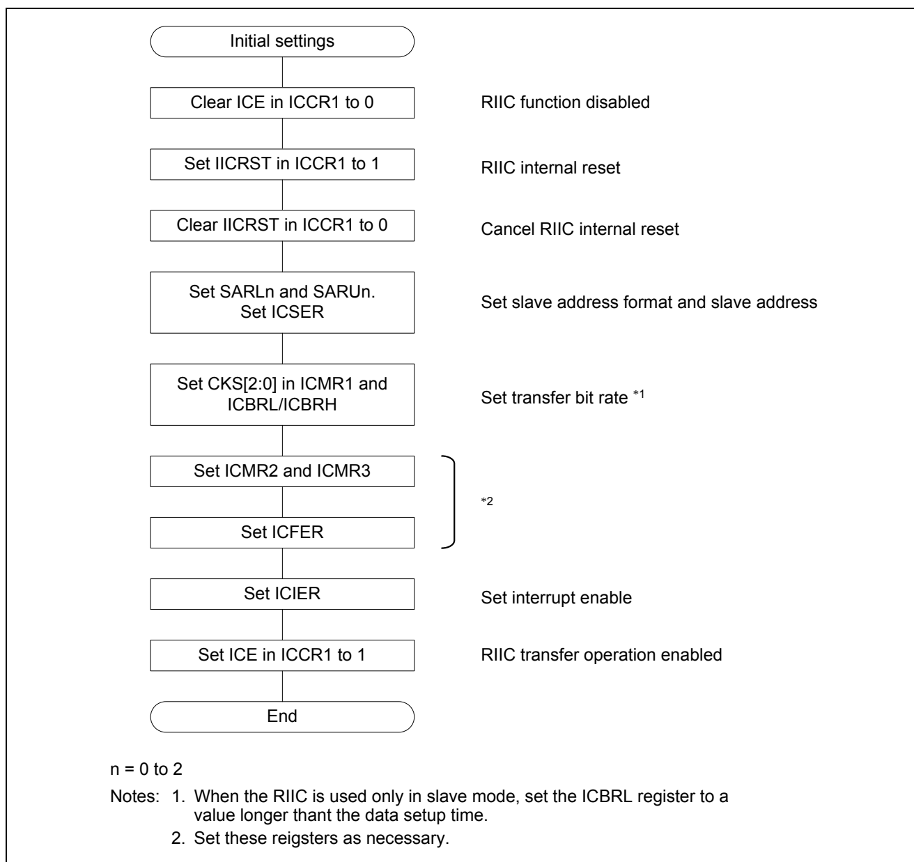
Figure 22.5 Example of RIIC Initialization Flow
