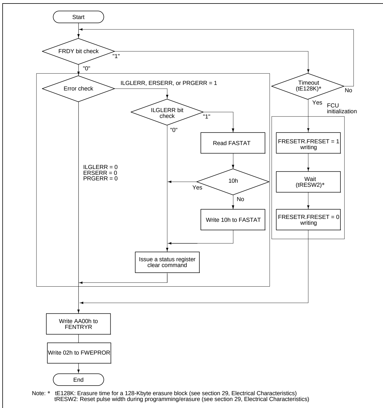
Figure 26.7 Procedure for Transition to ROM Read Mode
