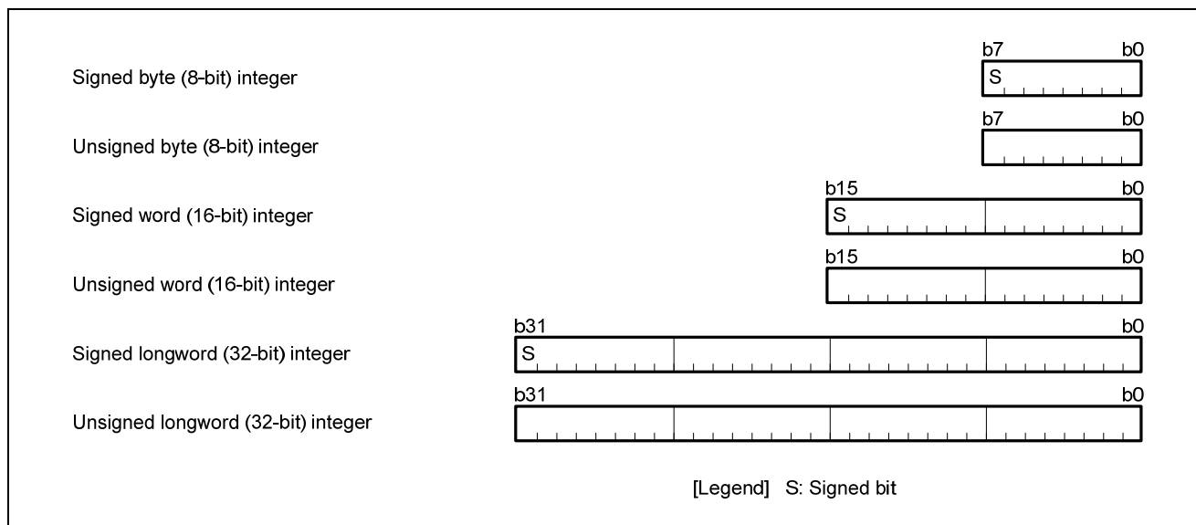
Figure 2.2 Integer
