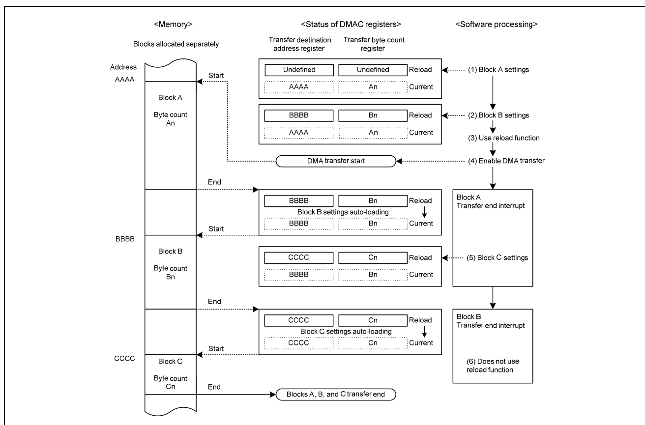
Figure 12.6 Example of DMA Transfer Using the Reload Function
