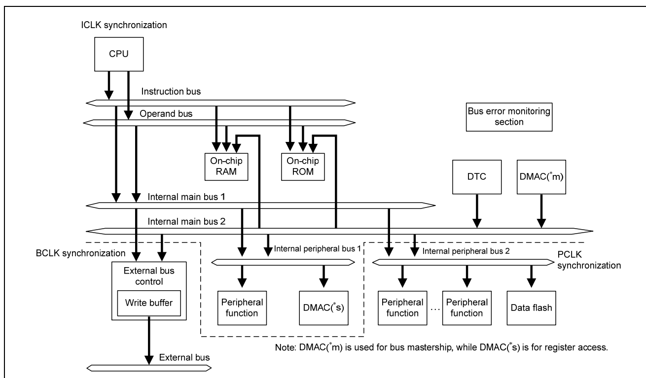
Figure 11.1 Bus Configuration
