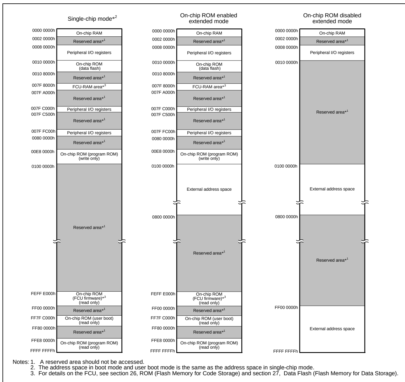
Figure 4.2 Memory Map of the R5F56107
