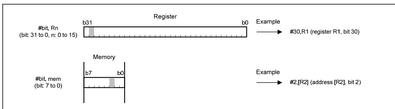
Figure 2.4 Bit
