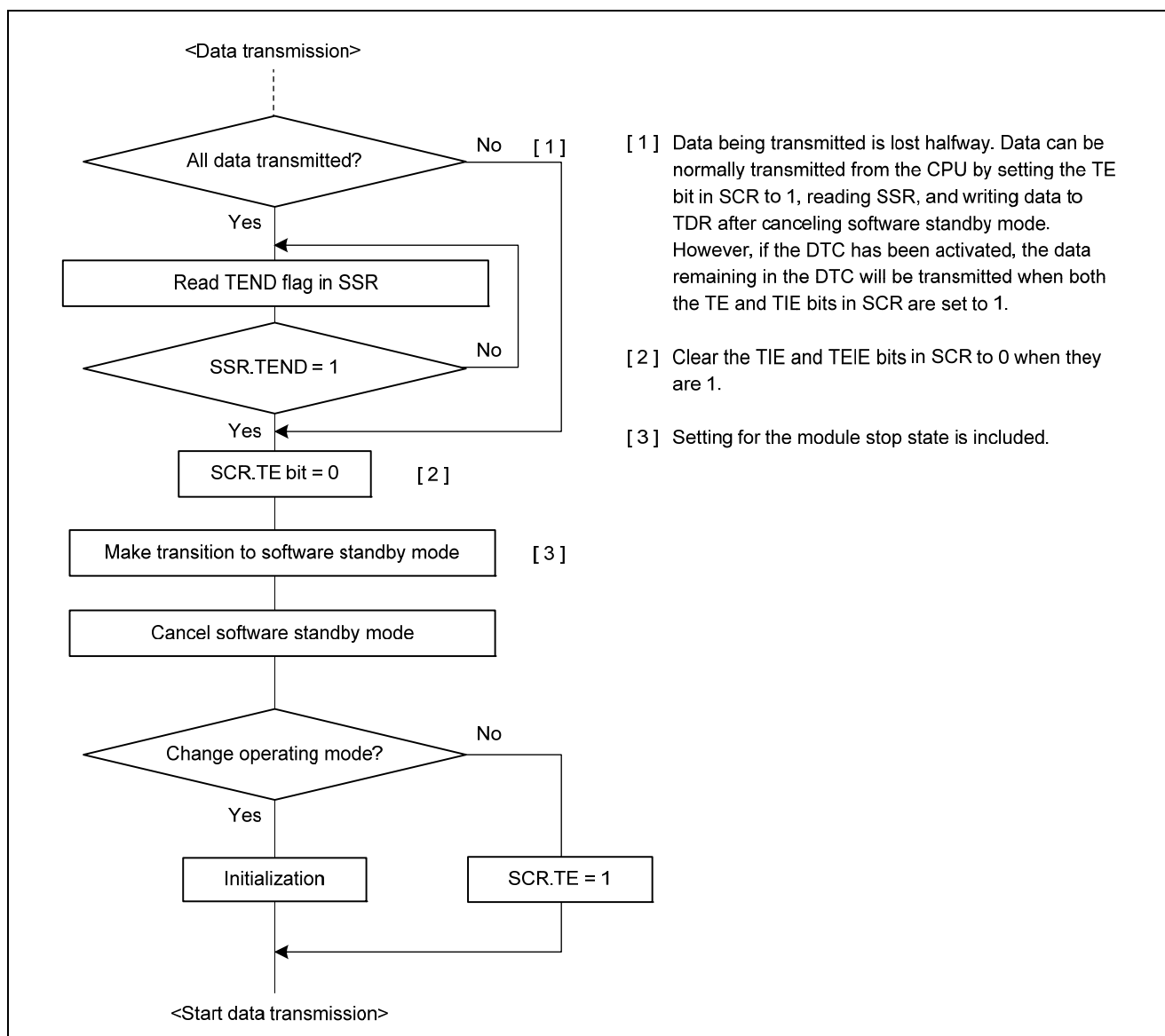
Figure 20.31 Example of Flowchart for Transition to Software Standby Mode during Transmission
