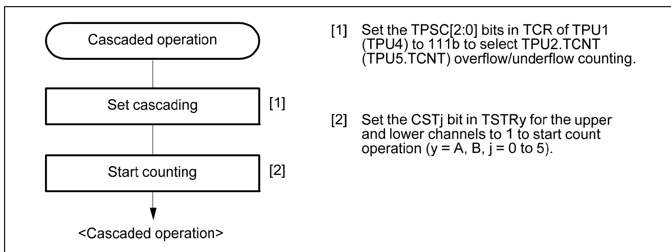
Figure 15.18 Cascaded Operation Setting Procedure
