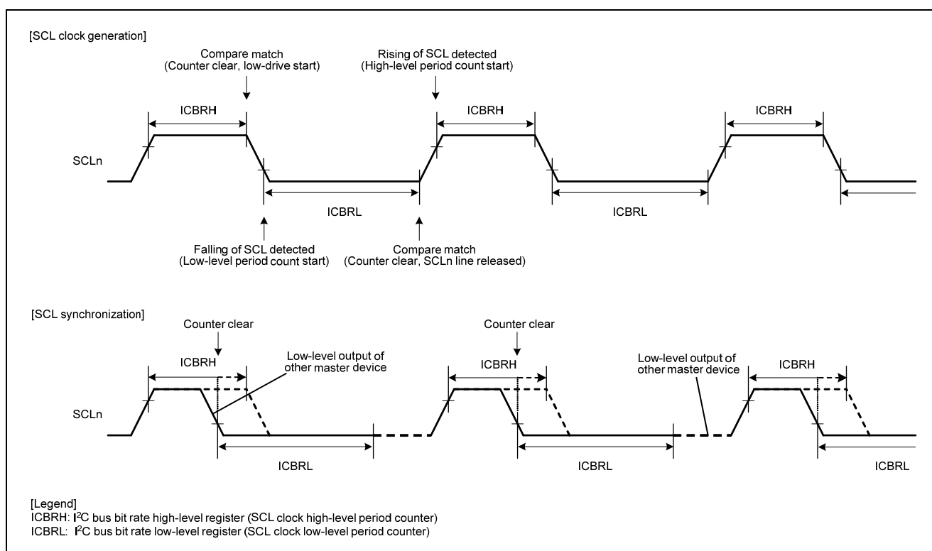
Figure 22.20 Generation and Synchronization of the SCL Signal from the RIIC
