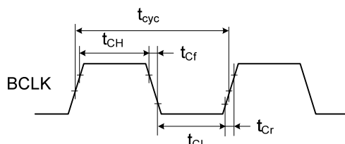
Figure 29.1 External Bus Clock Timing
