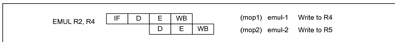
Figure 2.16 EMUL, EMULU Instructions (Register- Register, Register-Immediate)
