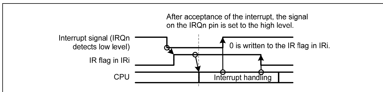
Figure 10.6 Operation of the IR Flag in IRI in the Case of Level Detection of an External Interrupt
