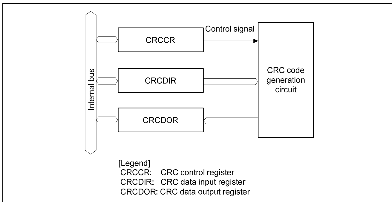
Figure 21.1 Block Diagram of CRC Calculator
