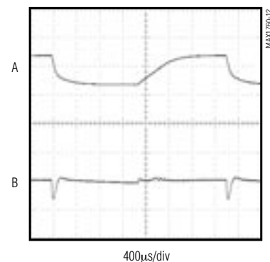
LINE-TRANSIENT RESPONSE
