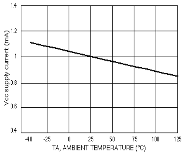
Figure 8. ICC Supply Current versus Temperature
