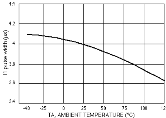
Figure 23. I1 Pulse Current Width versus Temperature
