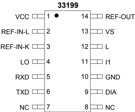
Figure 3. 33199 Pin Connections
