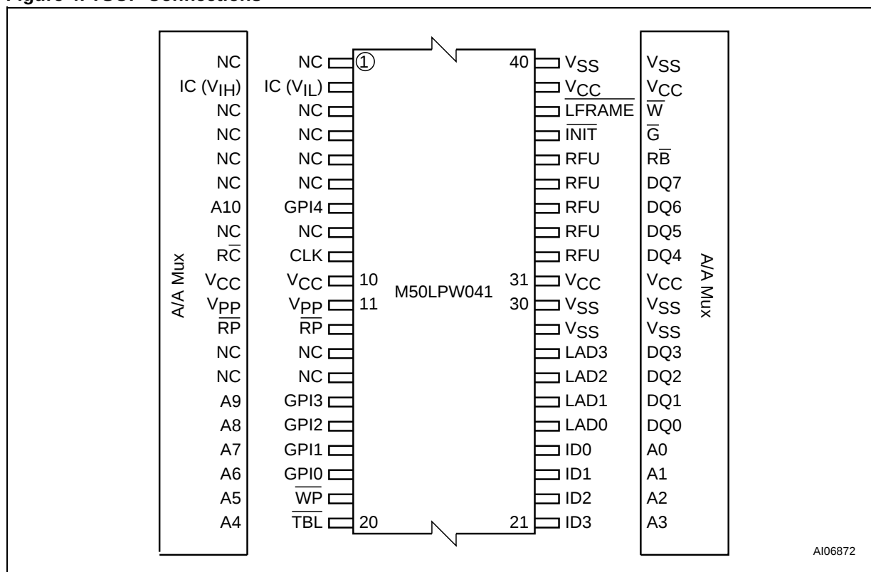
Figure 4. TSOP Connections
