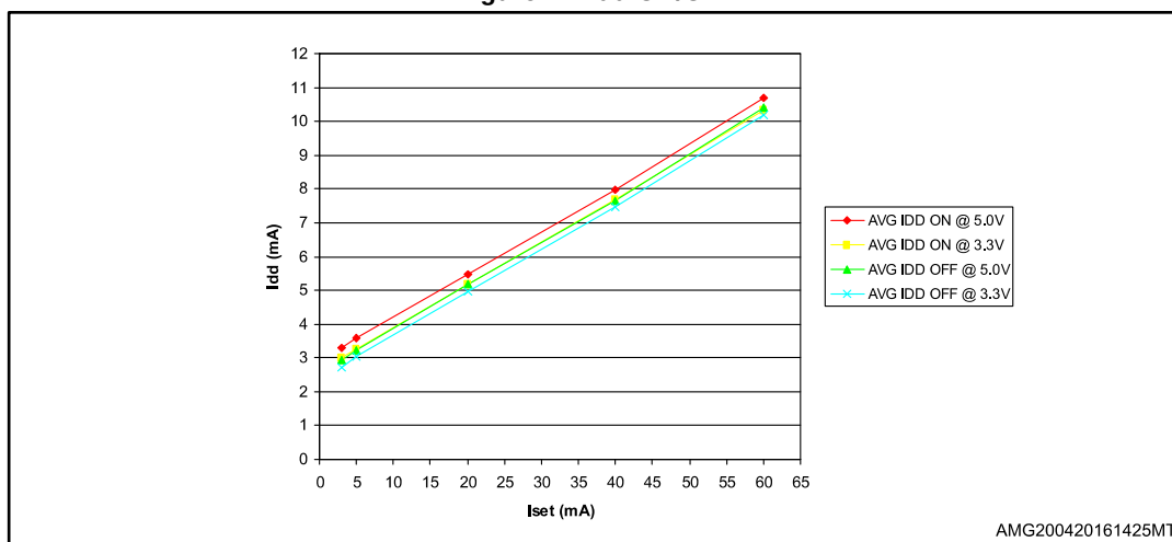
Figure 14: I_{DD} ON/OFF
