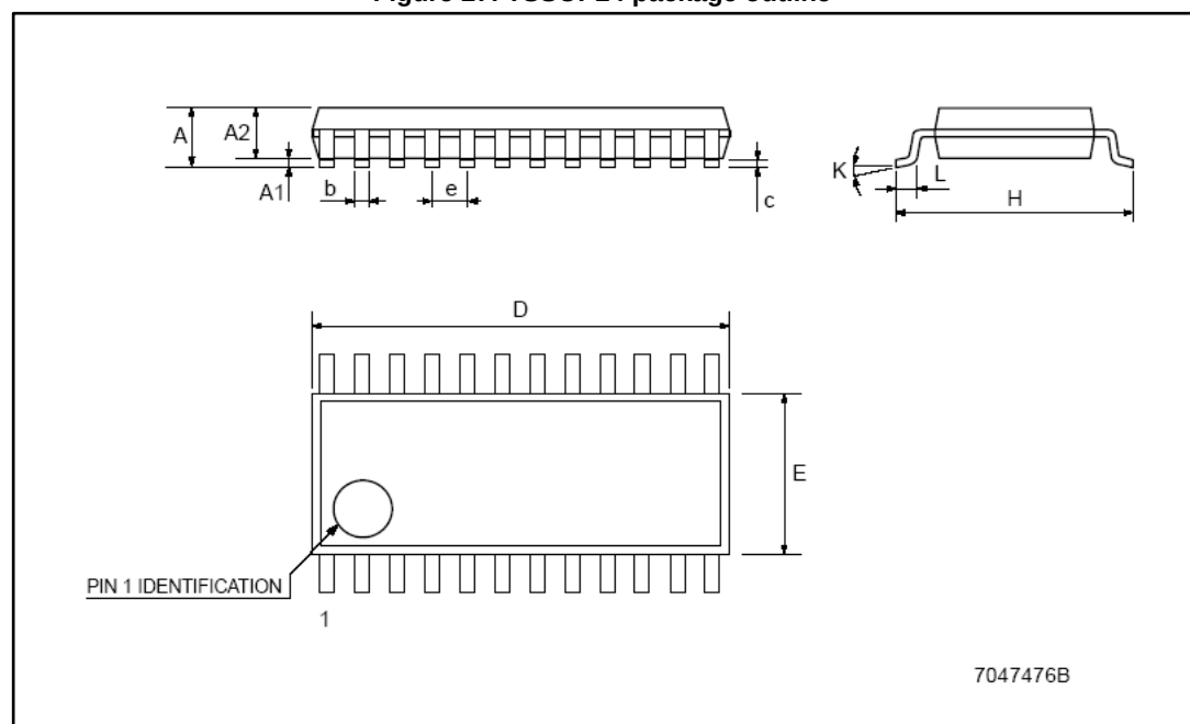
Figure 27: TSSOP24 package outline
