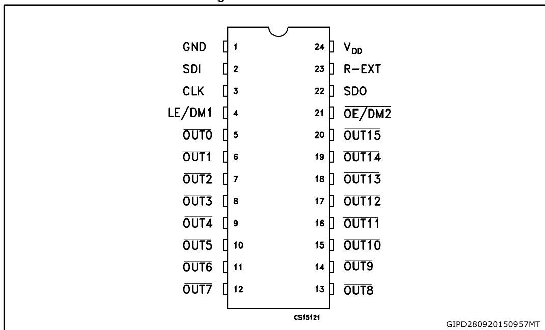
Figure 1: Pin connection
