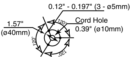
Mounting Hole Layout: Base Mounting Style
