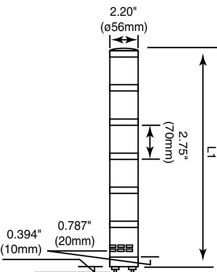
Assembled Base Mount
