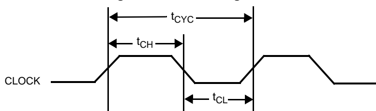
Figure 49. Clock Timing
