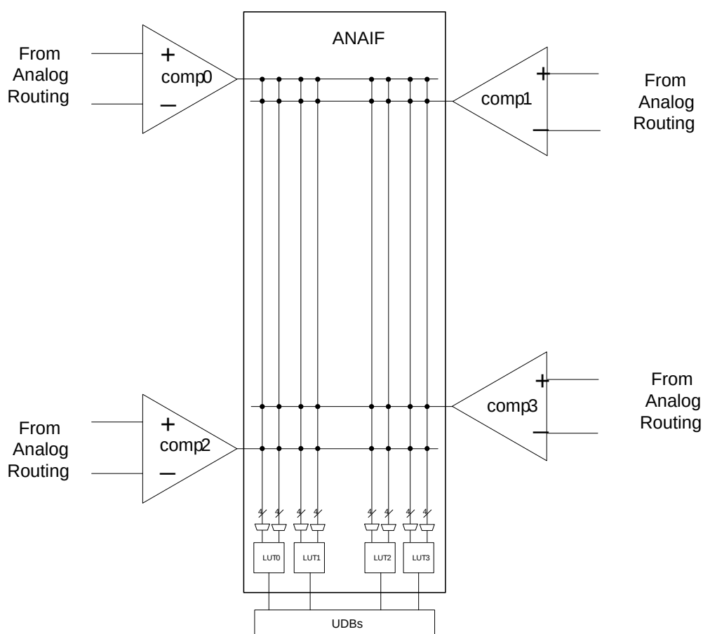
Figure 8-4. Analog Comparator
