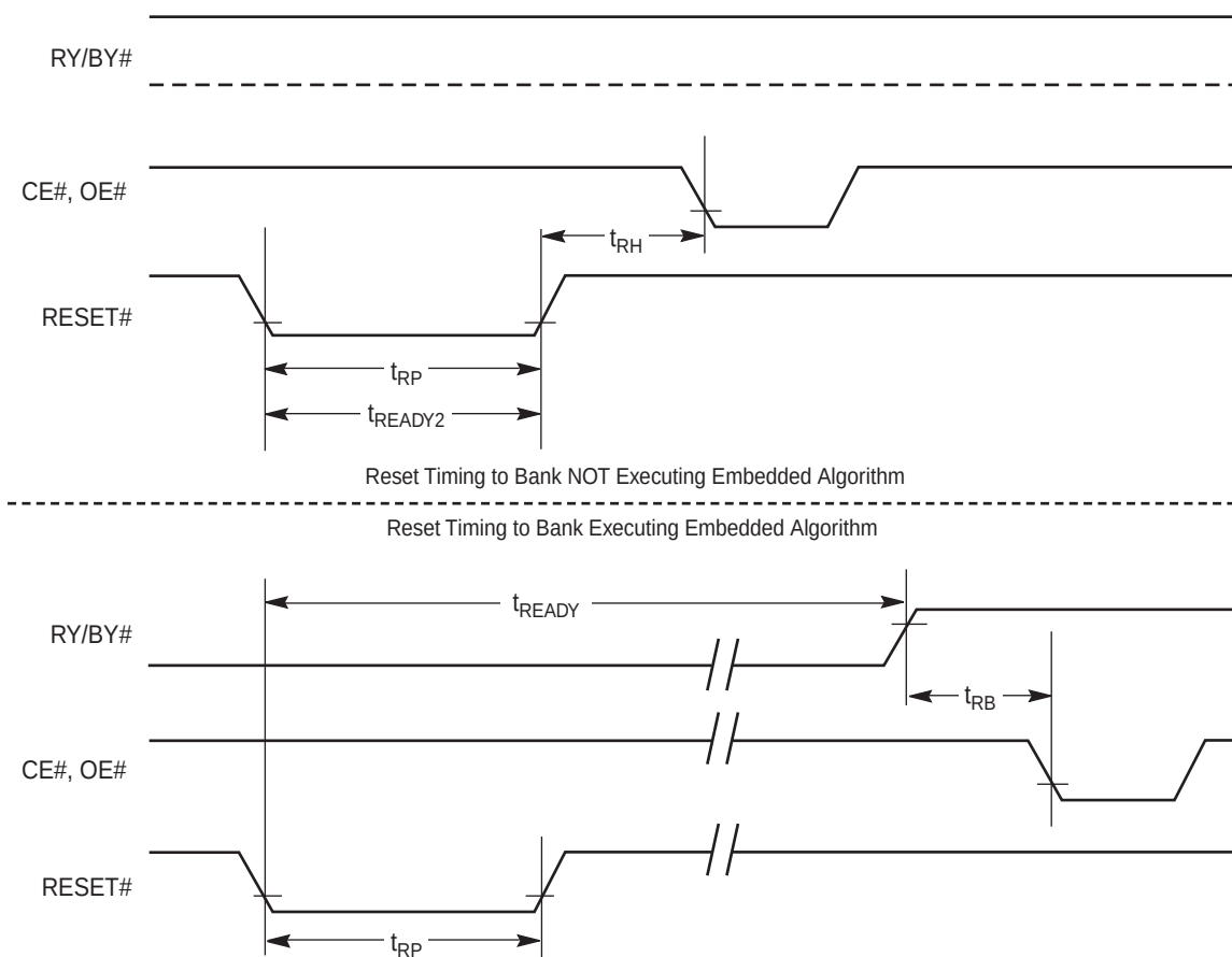
Figure 18.6 RESET# Timings
