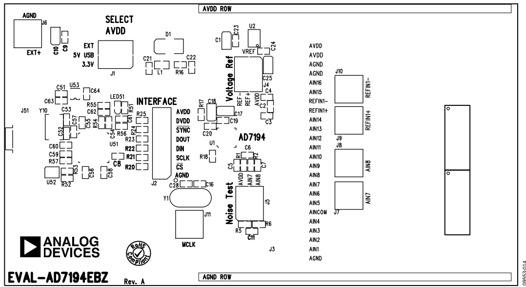
Figure 14. EVAL-AD7194EBZ Silkscreen
