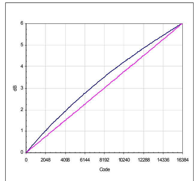
FIGURE 5B. ISL5416 AGC FORWARD GAIN RESPONSE MAGNIFIED VIEW (ACTUAL AND IDEAL LINEAR IN dB)
