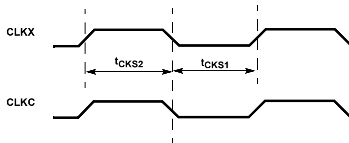
FIGURE 12. CLOCK SKEWS
