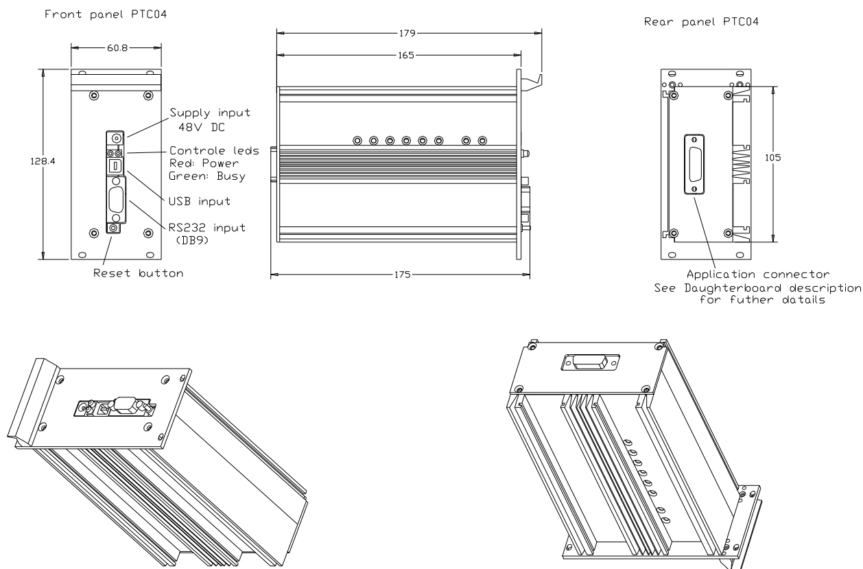
Figure 21-1: Mechanical Outlines
