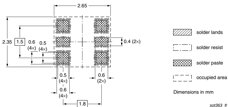
Fig 12. Reflow soldering footprint BAV99S (SOT363/SC-88)
