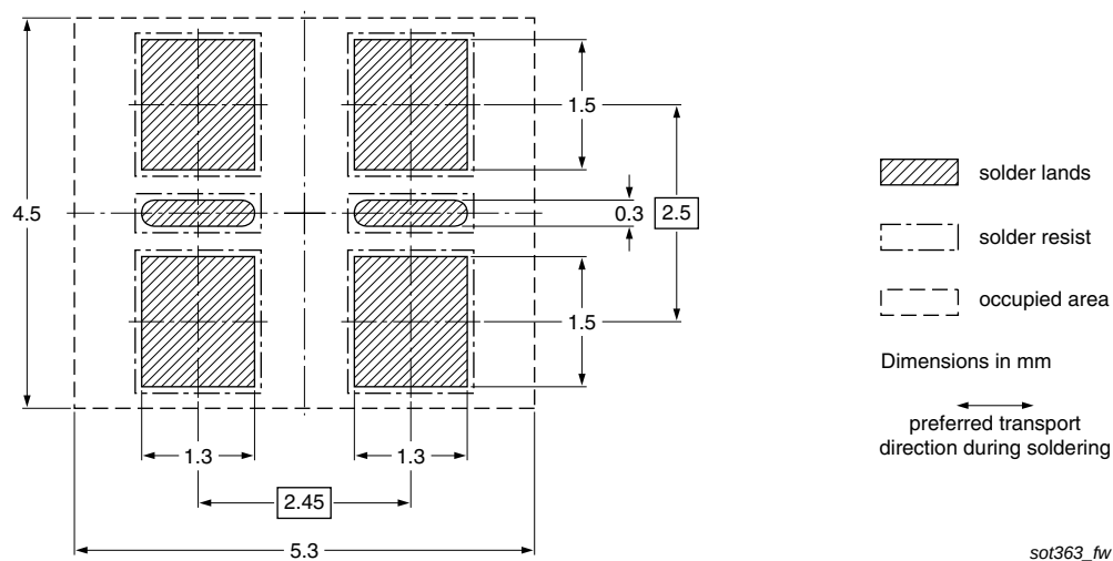
Fig 13. Wave soldering footprint BAV99S (SOT363/SC-88)
