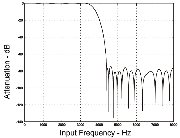
Figure 5. FIR Transmit Filter Response
