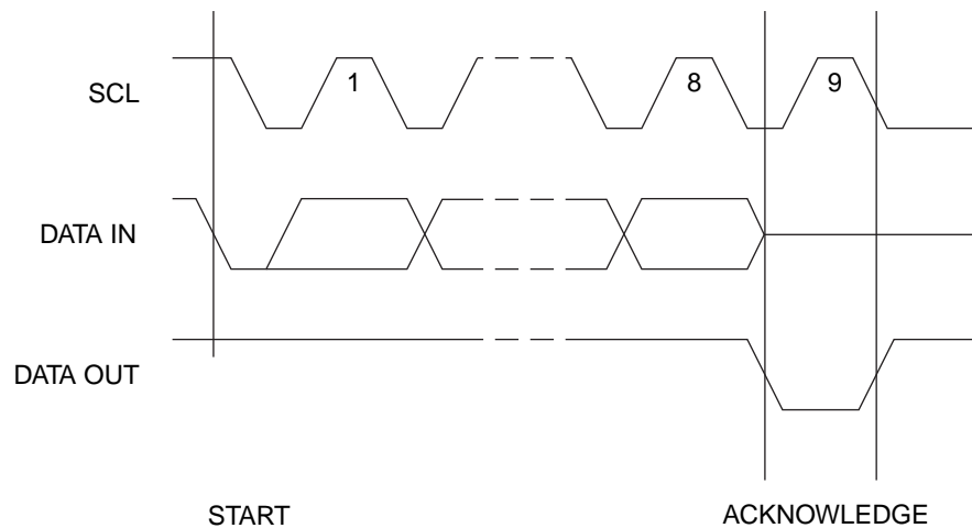
Figure 5-5. Output Acknowledge
