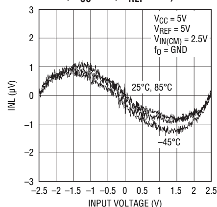
Integral Nonlinearity (2x Speed Mode; V_{\text{CC}} = 5\text{V} , V_{\text{REF}} = 5\text{V} )
