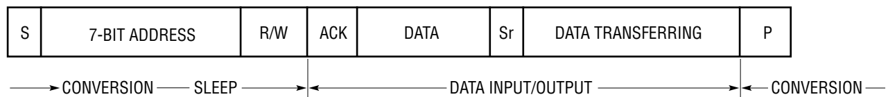
Figure 6. Conversion Sequence
