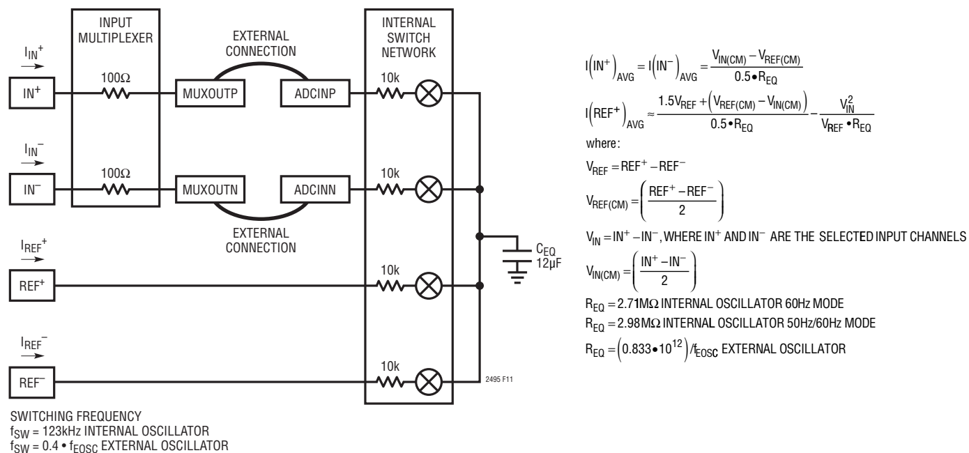
Figure 11. Equivalent Analog Input Circuit
