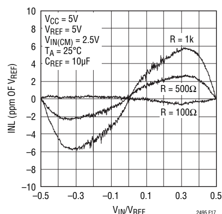
Figure 17. INL vs Differential Input Voltage and Reference Source Resistance for C_{REF} > 1\mu F
