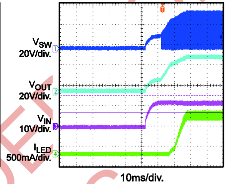
V_{in} Startup
