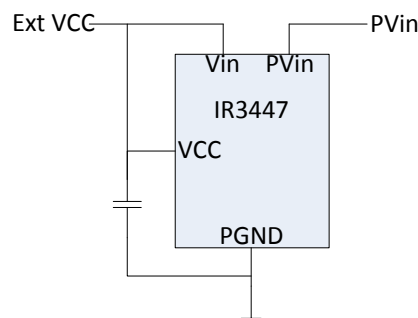
Figure 17: Externally Biased Configuration
