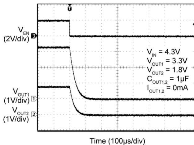
MIC5393 Turn-Off Time (Auto-Discharge)
