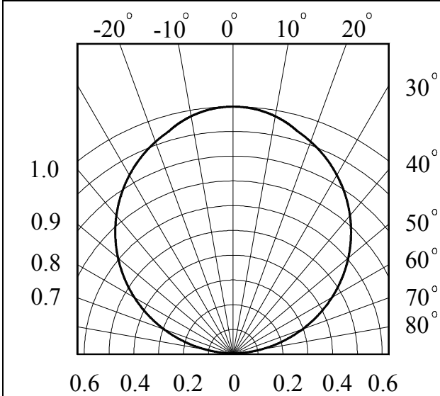
Relative Radiant Intensity vs. Angular Displacement (X-axis)
