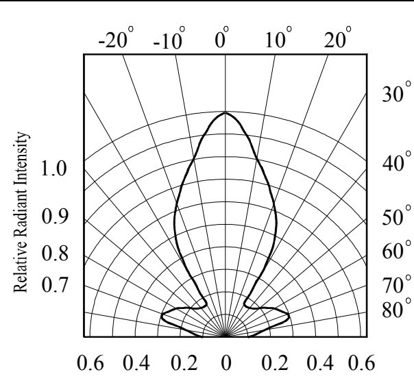
Relative Radiant Intensity vs. Angular Displacement (Y-axis)
